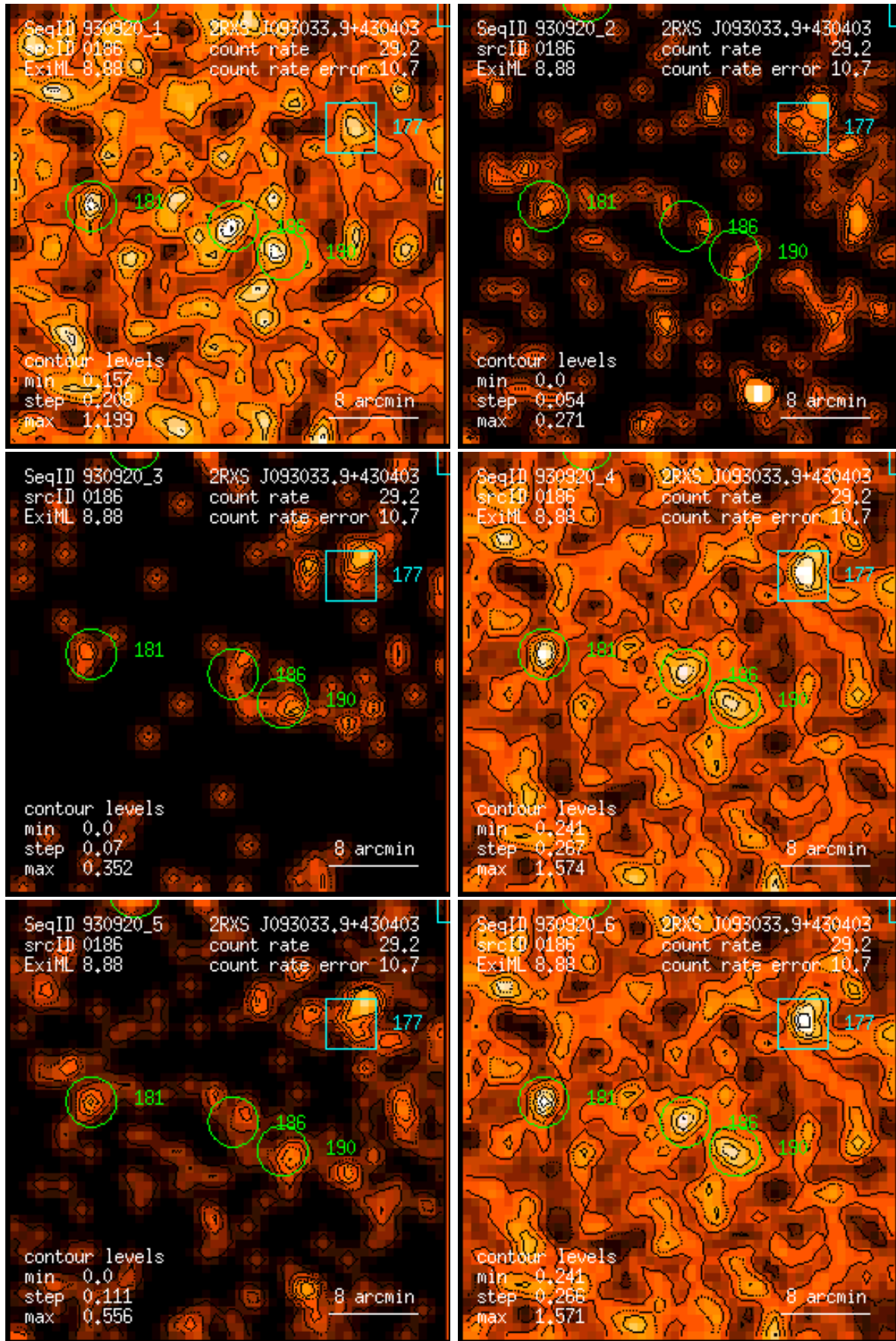
Figure 186: RASS 930920: detection 0186: band rate images, Gaussian filter: (1) PSPC channels 11 – 41, (2) 52 – 90, (3) 91 – 201, (4) 11 – 235, (5) 52 – 201, (6) 11 – 201. Broad band rates in counts/ks. Band rate contour levels in counts/ks/arcmin 2 .
