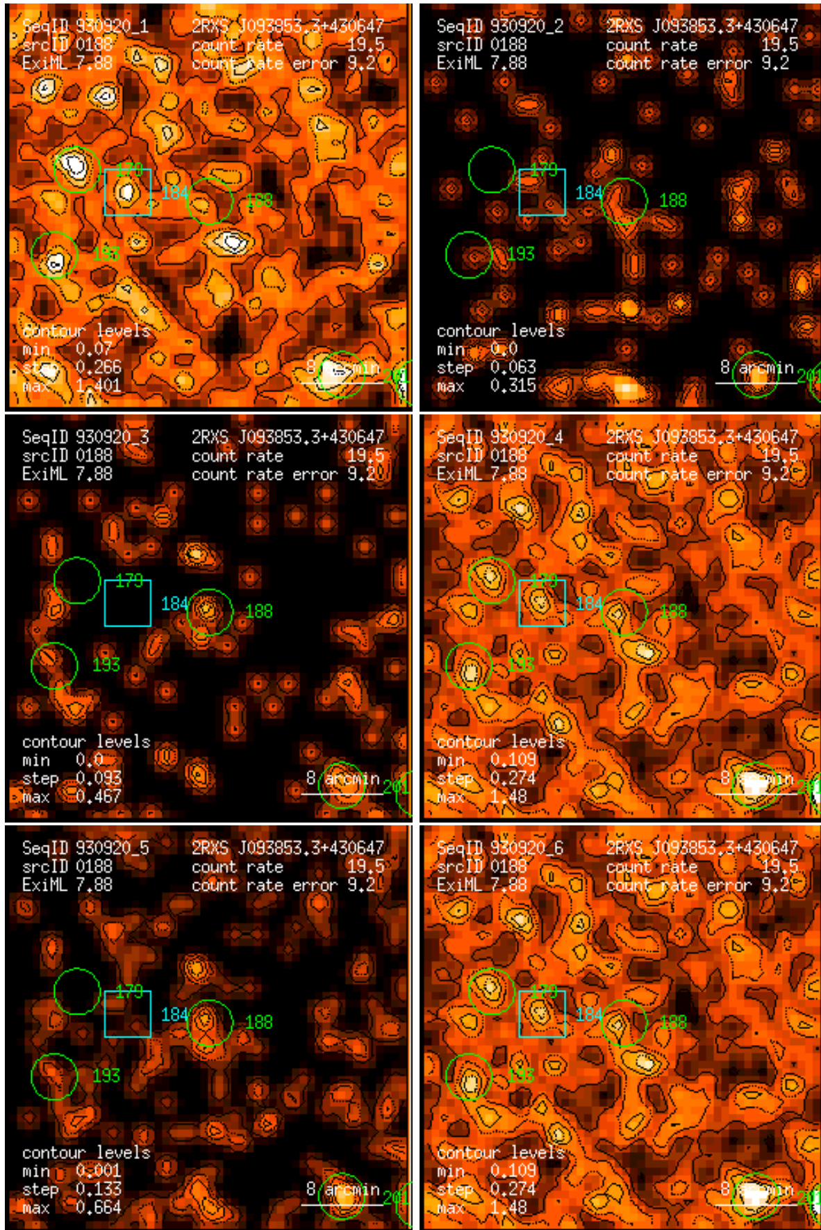
Figure 188: RASS 930920: detection 0188: band rate images, Gaussian filter: (1) PSPC channels 11 – 41, (2) 52 – 90, (3) 91 – 201, (4) 11 – 235, (5) 52 – 201, (6) 11 – 201. Broad band rates in counts/ks. Band rate contour levels in counts/ks/arcmin 2 .
