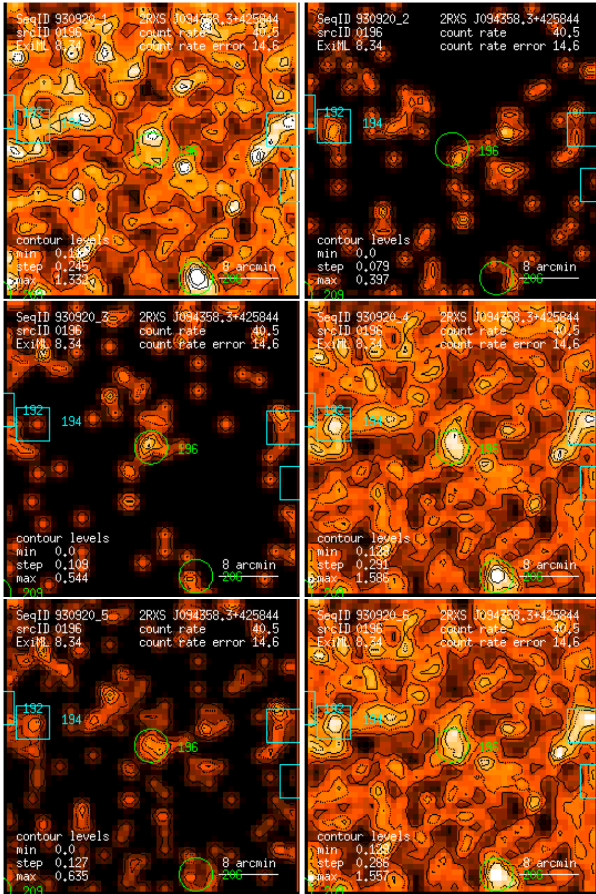
Figure 196: RASS 930920: detection 0196: band rate images, Gaussian filter: (1) PSPC channels 11 – 41, (2) 52 – 90, (3) 91 – 201, (4) 11 – 235, (5) 52 – 201, (6) 11 – 201. Broad band rates in counts/ks. Band rate contour levels in counts/ks/arcmin 2 .
