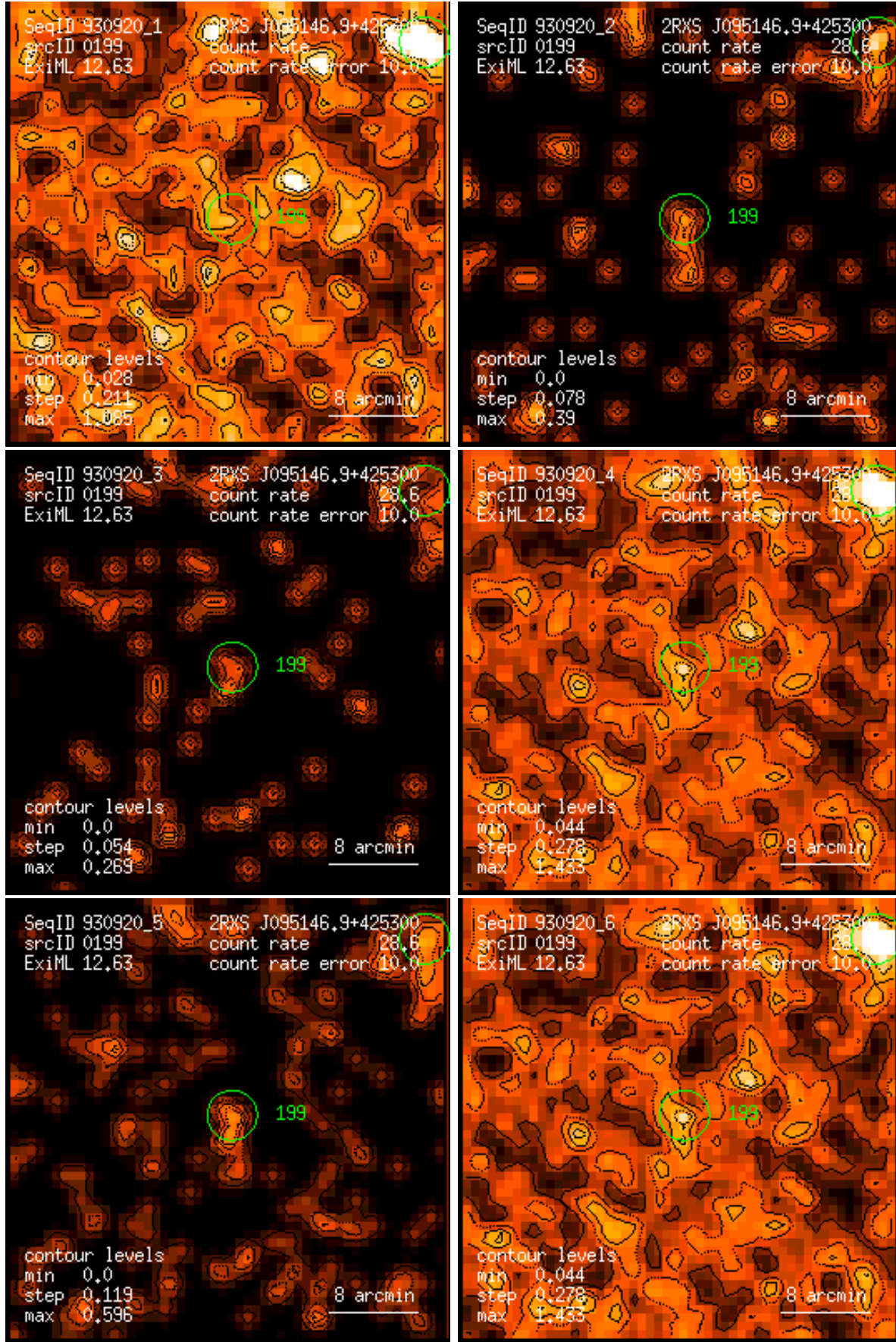
Figure 199: RASS 930920: detection 0199: band rate images, Gaussian filter: (1) PSPC channels 11 – 41, (2) 52 – 90, (3) 91 – 201, (4) 11 – 235, (5) 52 – 201, (6) 11 – 201. Broad band rates in counts/ks. Band rate contour levels in counts/ks/arcmin 2 .
