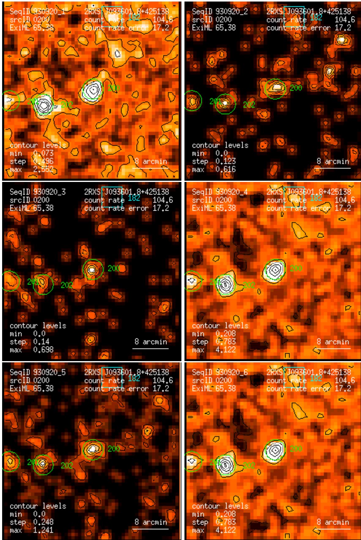
Figure 200: RASS 930920: detection 0200: band rate images, Gaussian filter: (1) PSPC channels 11 – 41, (2) 52 – 90, (3) 91 – 201, (4) 11 – 235, (5) 52 – 201, (6) 11 – 201. Broad band rates in counts/ks. Band rate contour levels in counts/ks/arcmin 2 .
