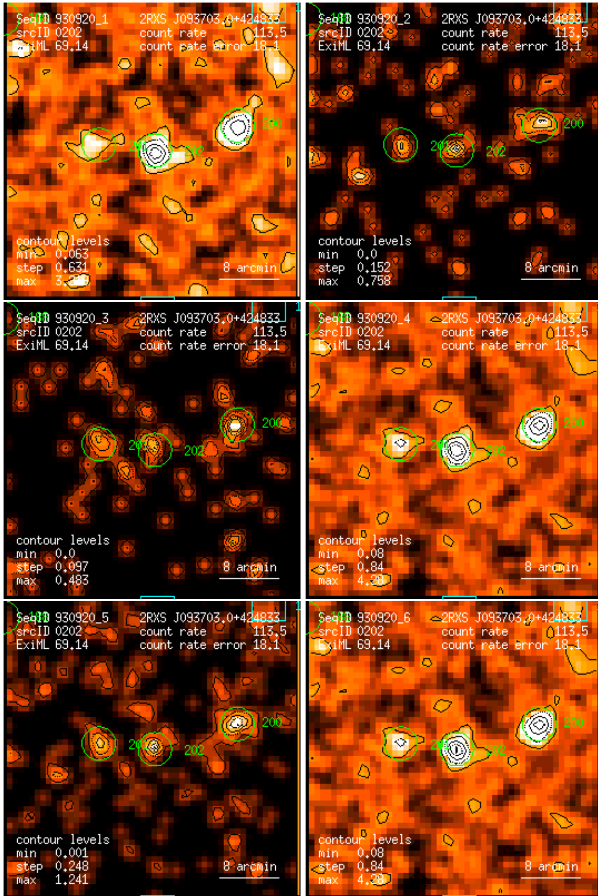
Figure 202: RASS 930920: detection 0202: band rate images, Gaussian filter: (1) PSPC channels 11 – 41, (2) 52 – 90, (3) 91 – 201, (4) 11 – 235, (5) 52 – 201, (6) 11 – 201. Broad band rates in counts/ks. Band rate contour levels in counts/ks/arcmin 2 .
