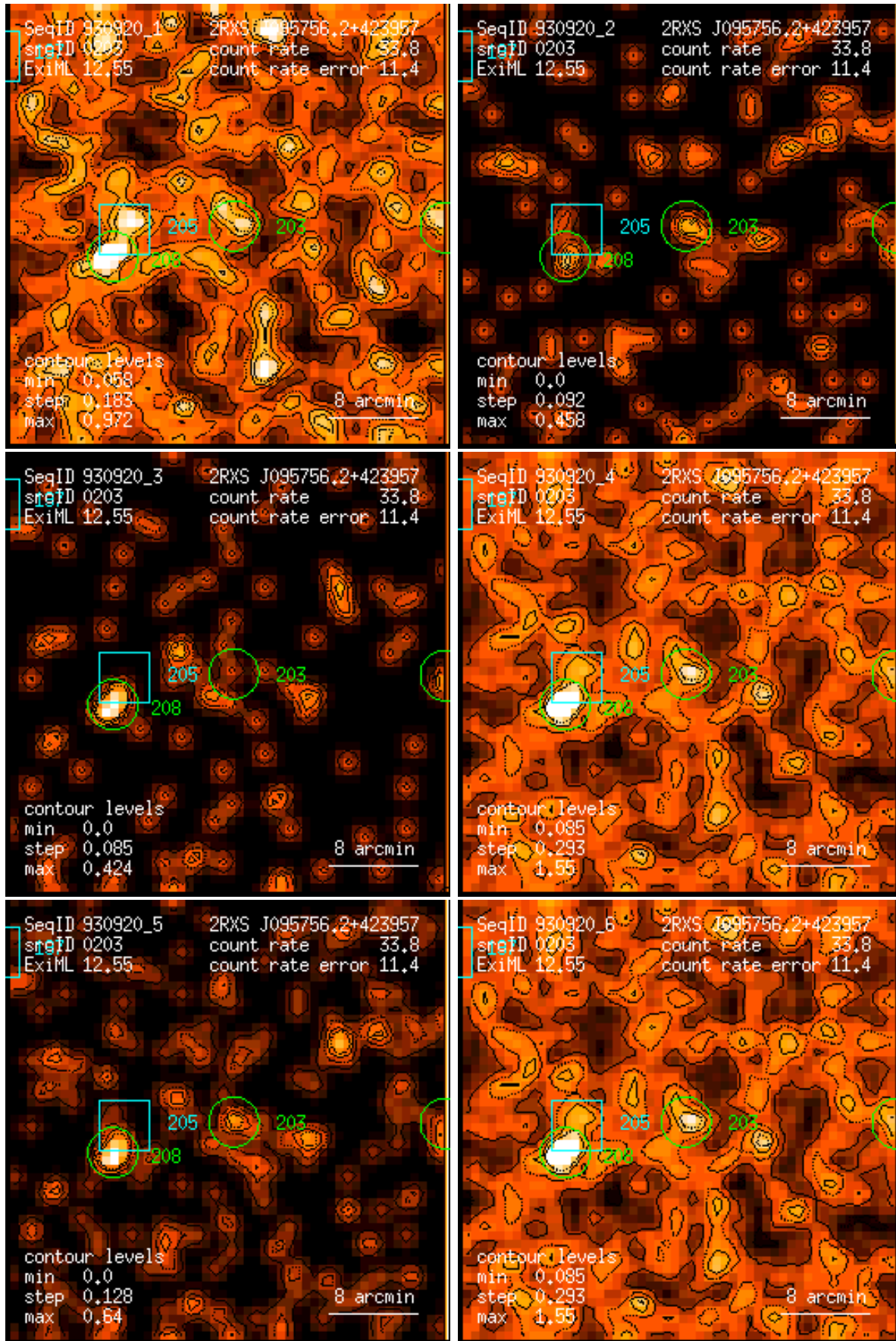
Figure 203: RASS 930920: detection 0203: band rate images, Gaussian filter: (1) PSPC channels 11 – 41, (2) 52 – 90, (3) 91 – 201, (4) 11 – 235, (5) 52 – 201, (6) 11 – 201. Broad band rates in counts/ks. Band rate contour levels in counts/ks/arcmin 2 .
