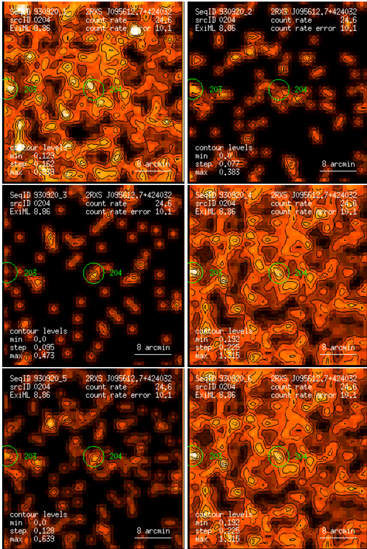
Figure 204: RASS 930920: detection 0204: band rate images, Gaussian filter: (1) PSPC channels 11 – 41, (2) 52 – 90, (3) 91 – 201, (4) 11 – 235, (5) 52 – 201, (6) 11 – 201. Broad band rates in counts/ks. Band rate contour levels in counts/ks/arcmin 2 .
