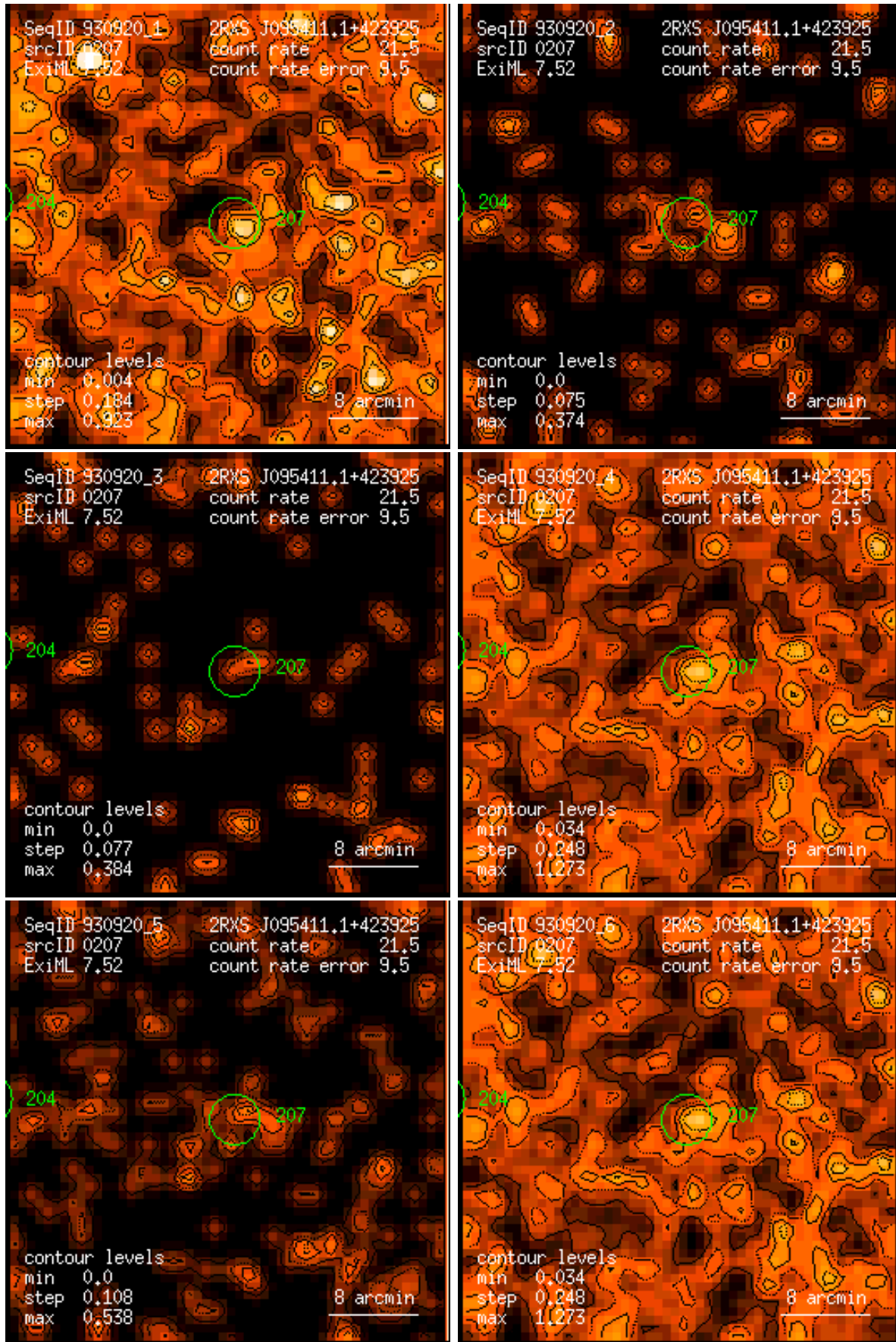
Figure 207: RASS 930920: detection 0207: band rate images, Gaussian filter: (1) PSPC channels 11 – 41, (2) 52 – 90, (3) 91 – 201, (4) 11 – 235, (5) 52 – 201, (6) 11 – 201. Broad band rates in counts/ks. Band rate contour levels in counts/ks/arcmin 2 .
