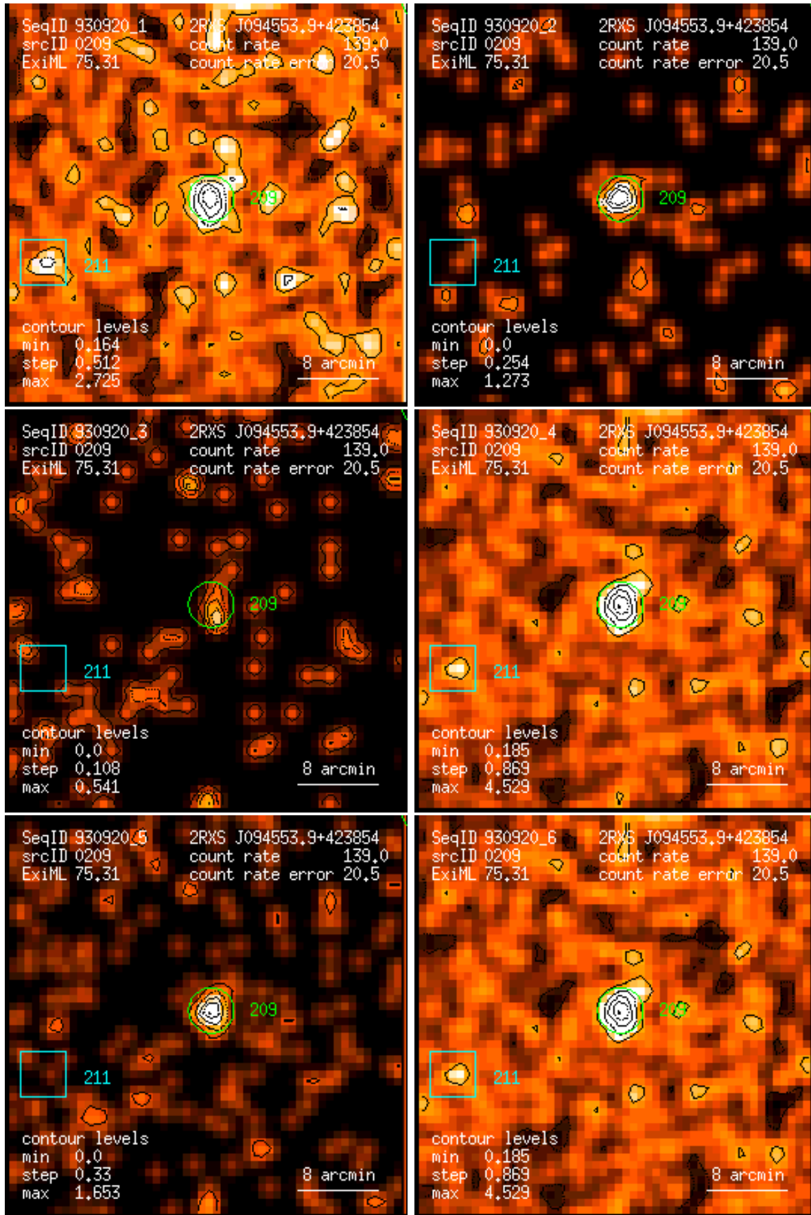
Figure 209: RASS 930920: detection 0209: band rate images, Gaussian filter: (1) PSPC channels 11 – 41, (2) 52 – 90, (3) 91 – 201, (4) 11 – 235, (5) 52 – 201, (6) 11 – 201. Broad band rates in counts/ks. Band rate contour levels in counts/ks/arcmin 2 .
