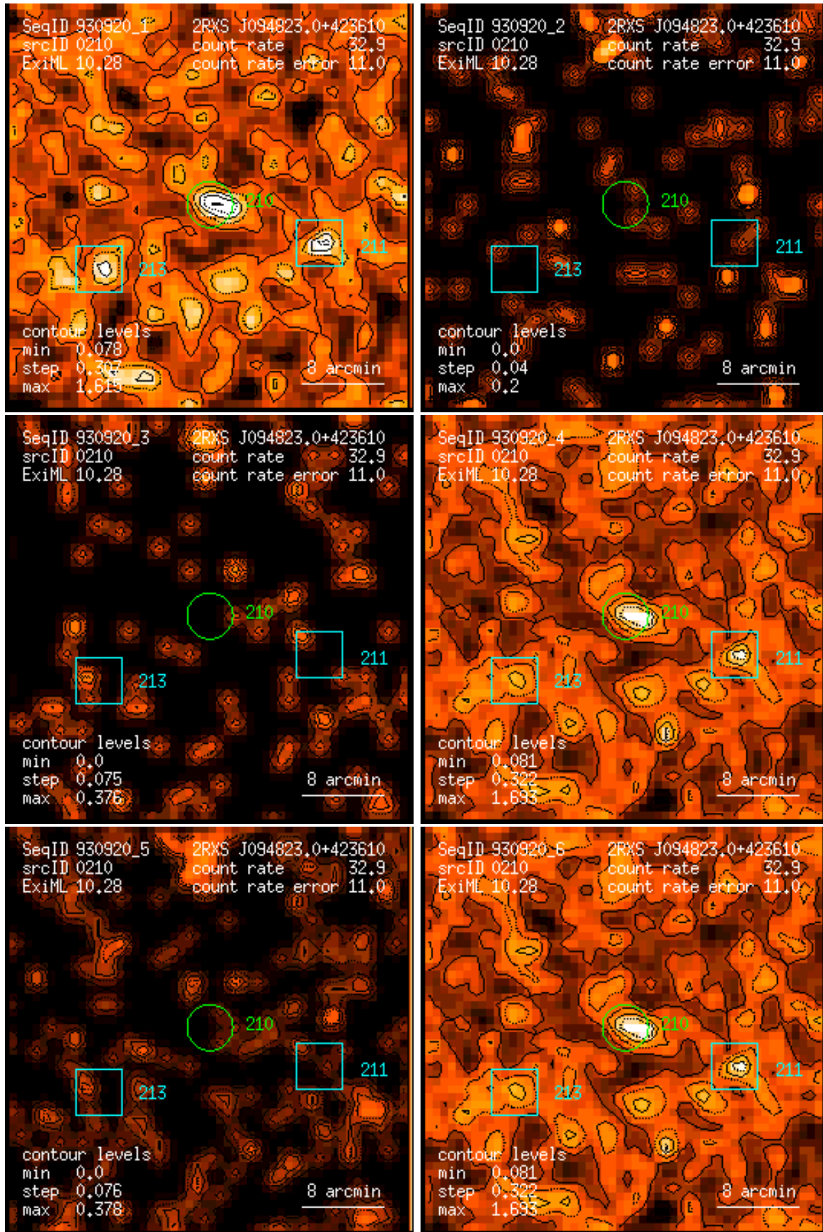
Figure 210: RASS 930920: detection 0210: band rate images, Gaussian filter: (1) PSPC channels 11 – 41, (2) 52 – 90, (3) 91 – 201, (4) 11 – 235, (5) 52 – 201, (6) 11 – 201. Broad band rates in counts/ks. Band rate contour levels in counts/ks/arcmin 2 .
