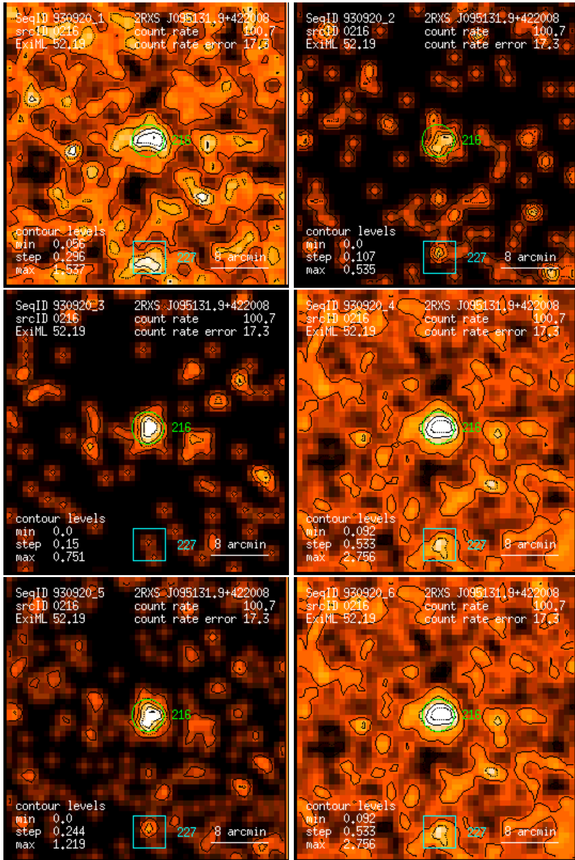
Figure 216: RASS 930920: detection 0216: band rate images, Gaussian filter: (1) PSPC channels 11 – 41, (2) 52 – 90, (3) 91 – 201, (4) 11 – 235, (5) 52 – 201, (6) 11 – 201. Broad band rates in counts/ks. Band rate contour levels in counts/ks/arcmin 2 .
