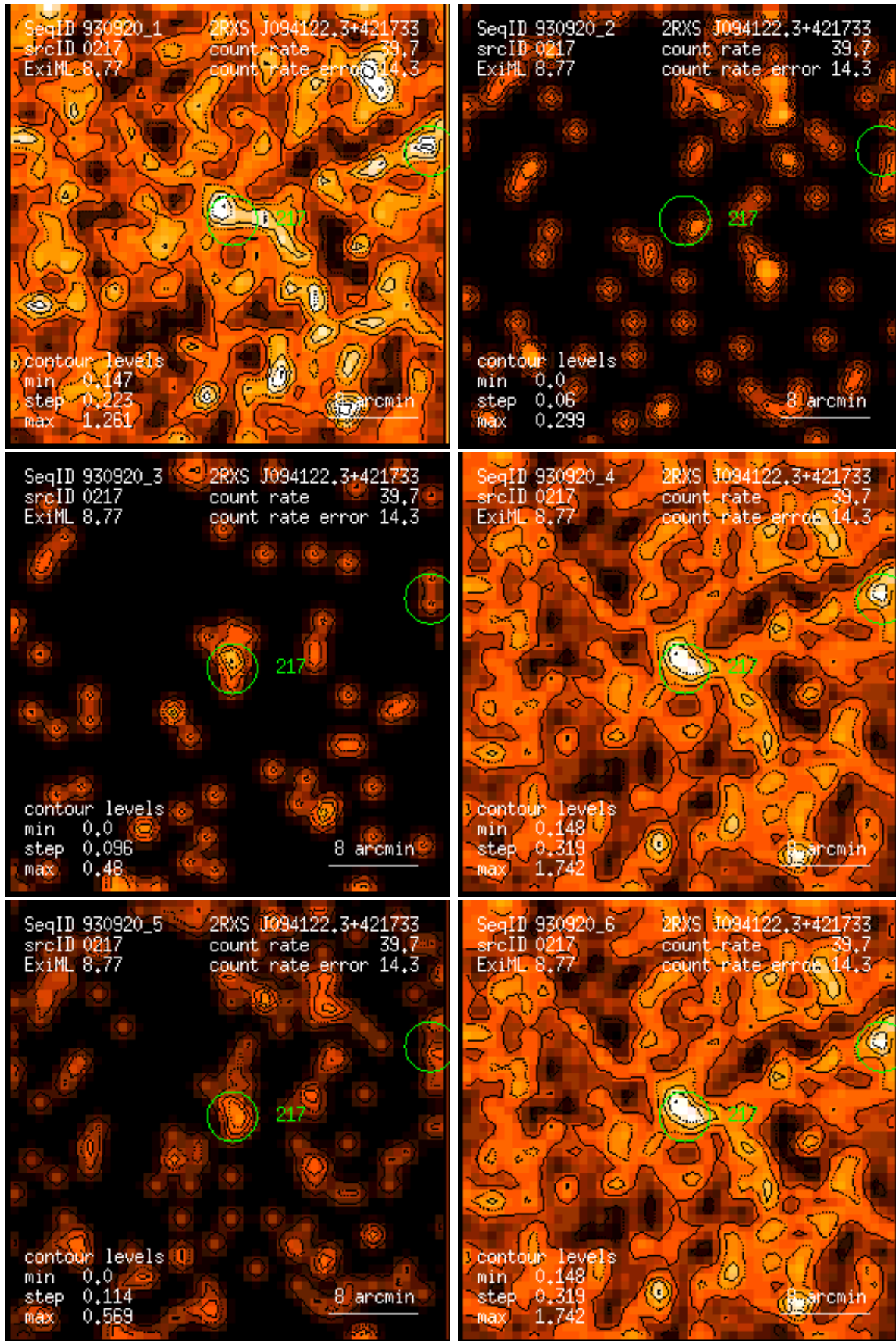
Figure 217: RASS 930920: detection 0217: band rate images, Gaussian filter: (1) PSPC channels 11 – 41, (2) 52 – 90, (3) 91 – 201, (4) 11 – 235, (5) 52 – 201, (6) 11 – 201. Broad band rates in counts/ks. Band rate contour levels in counts/ks/arcmin 2 .
