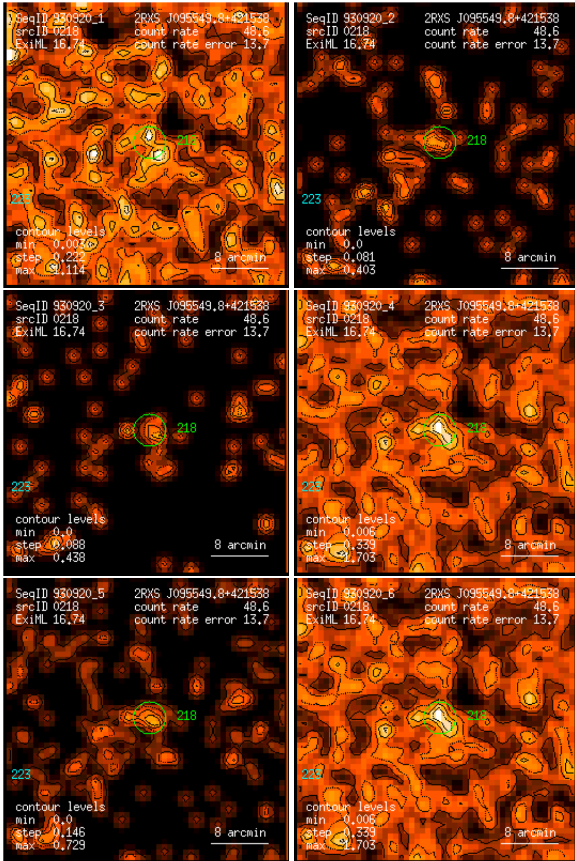
Figure 218: RASS 930920: detection 0218: band rate images, Gaussian filter: (1) PSPC channels 11 – 41, (2) 52 – 90, (3) 91 – 201, (4) 11 – 235, (5) 52 – 201, (6) 11 – 201. Broad band rates in counts/ks. Band rate contour levels in counts/ks/arcmin 2 .
