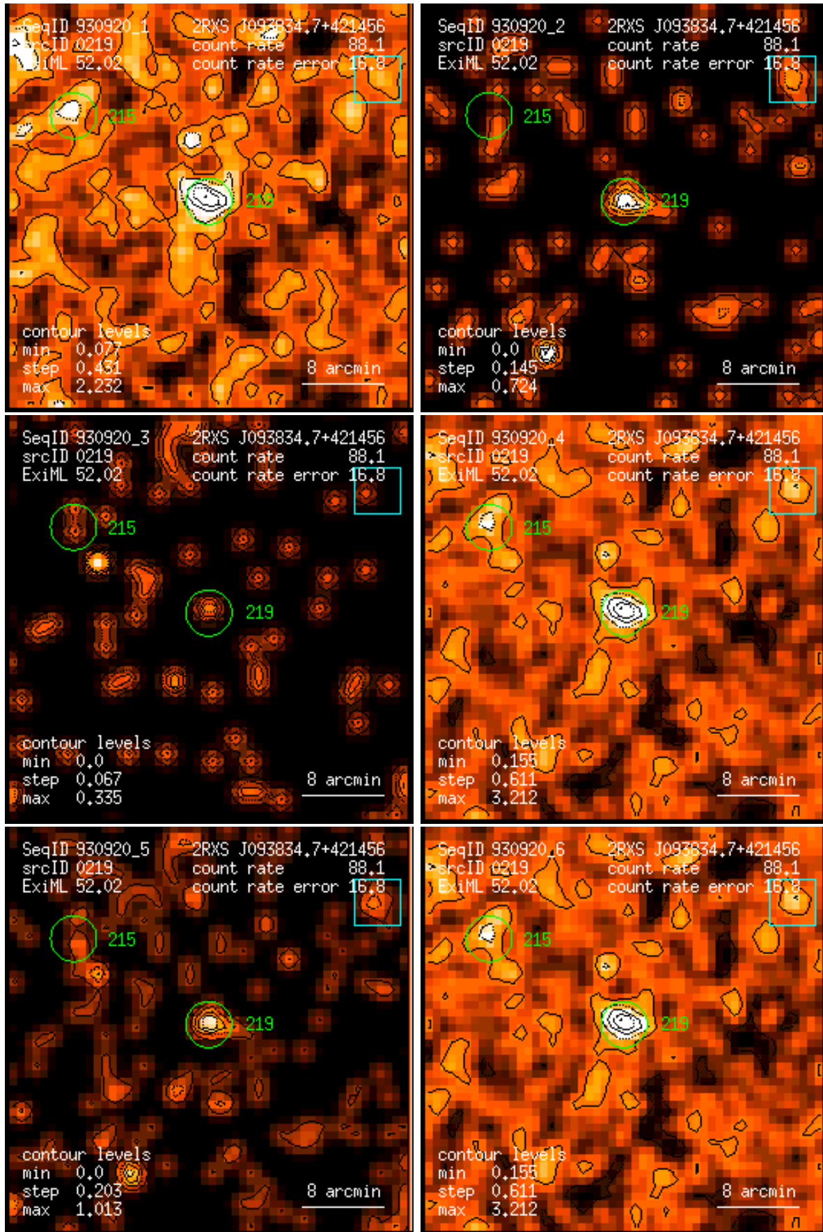
Figure 219: RASS 930920: detection 0219: band rate images, Gaussian filter: (1) PSPC channels 11 – 41, (2) 52 – 90, (3) 91 – 201, (4) 11 – 235, (5) 52 – 201, (6) 11 – 201. Broad band rates in counts/ks. Band rate contour levels in counts/ks/arcmin 2 .
