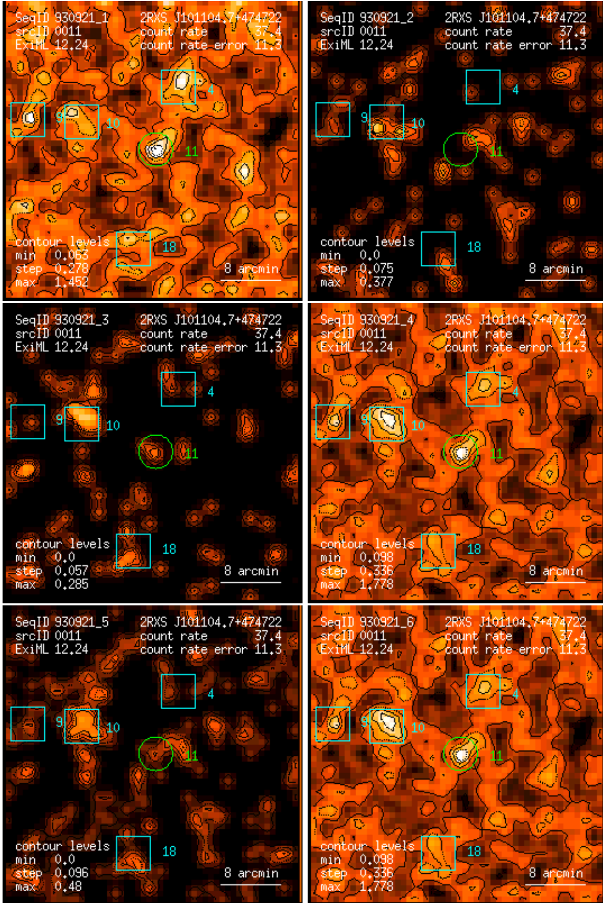
Figure 11: RASS 930921: detection 0011: band rate images, Gaussian filter: (1) PSPC channels 11 – 41, (2) 52 – 90, (3) 91 – 201, (4) 11 – 235, (5) 52 – 201, (6) 11 – 201. Broad band rates in counts/ks. Band rate contour levels in counts/ks/arcmin 2 .
