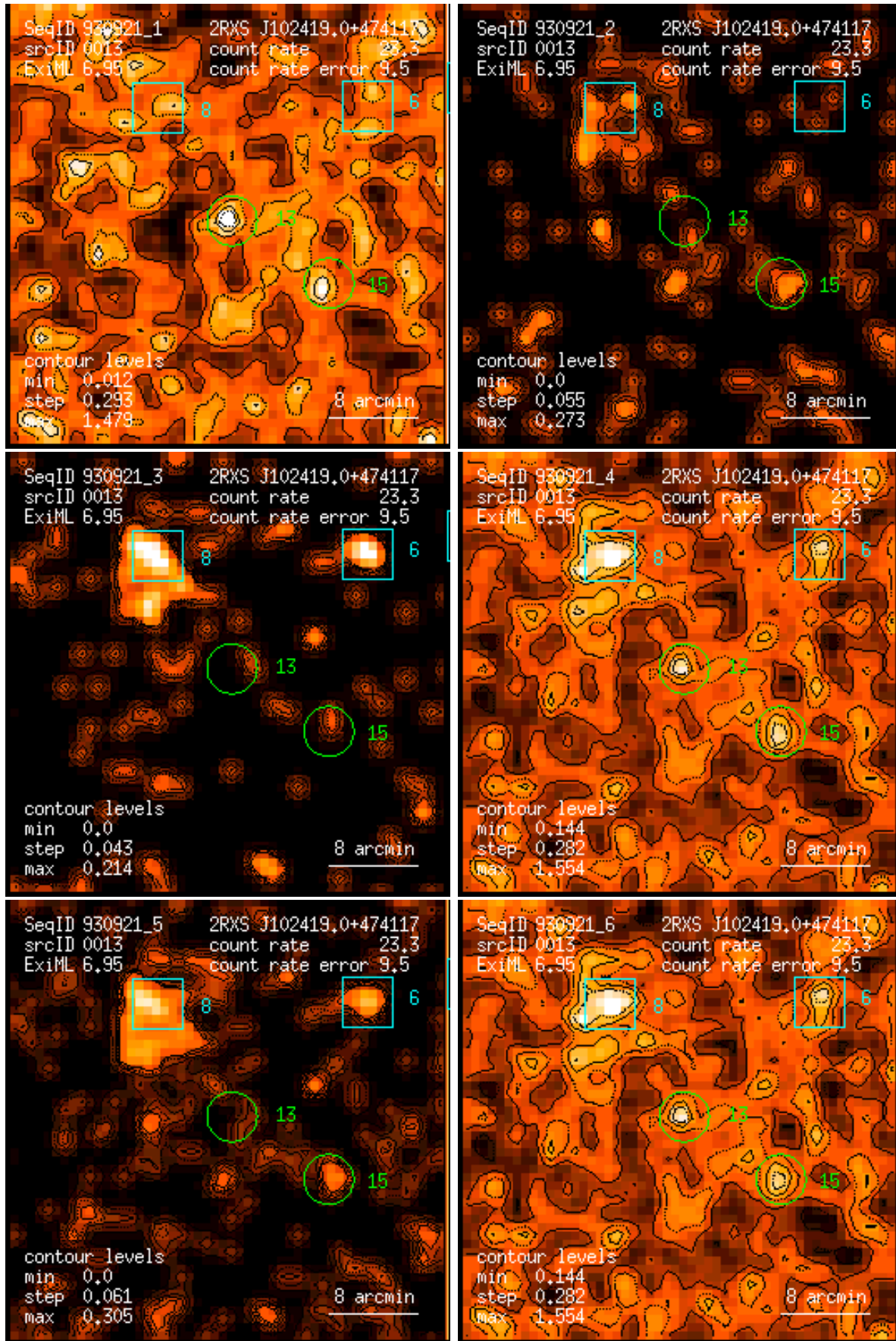
Figure 13: RASS 930921: detection 0013: band rate images, Gaussian filter: (1) PSPC channels 11 – 41, (2) 52 – 90, (3) 91 – 201, (4) 11 – 235, (5) 52 – 201, (6) 11 – 201. Broad band rates in counts/ks. Band rate contour levels in counts/ks/arcmin 2 .
