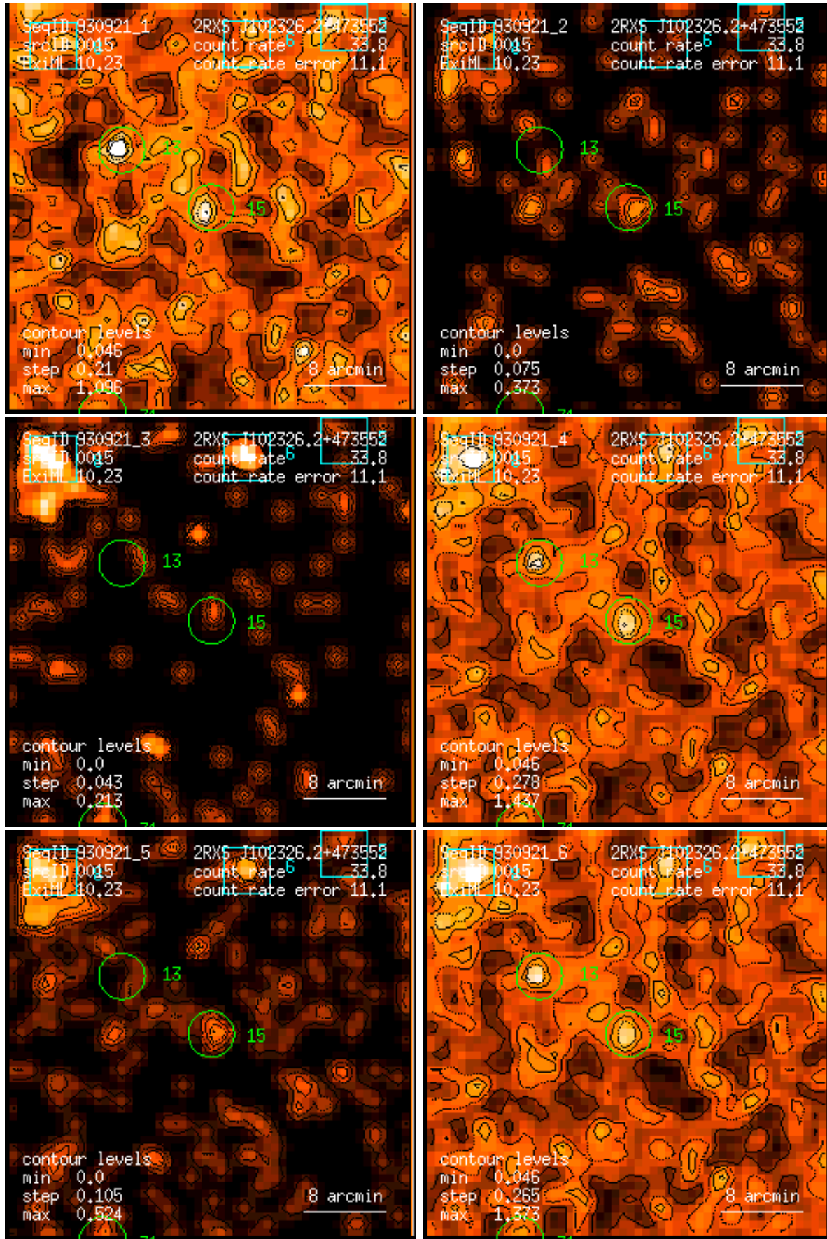
Figure 15: RASS 930921: detection 0015: band rate images, Gaussian filter: (1) PSPC channels 11 – 41, (2) 52 – 90, (3) 91 – 201, (4) 11 – 235, (5) 52 – 201, (6) 11 – 201. Broad band rates in counts/ks. Band rate contour levels in counts/ks/arcmin 2 .
