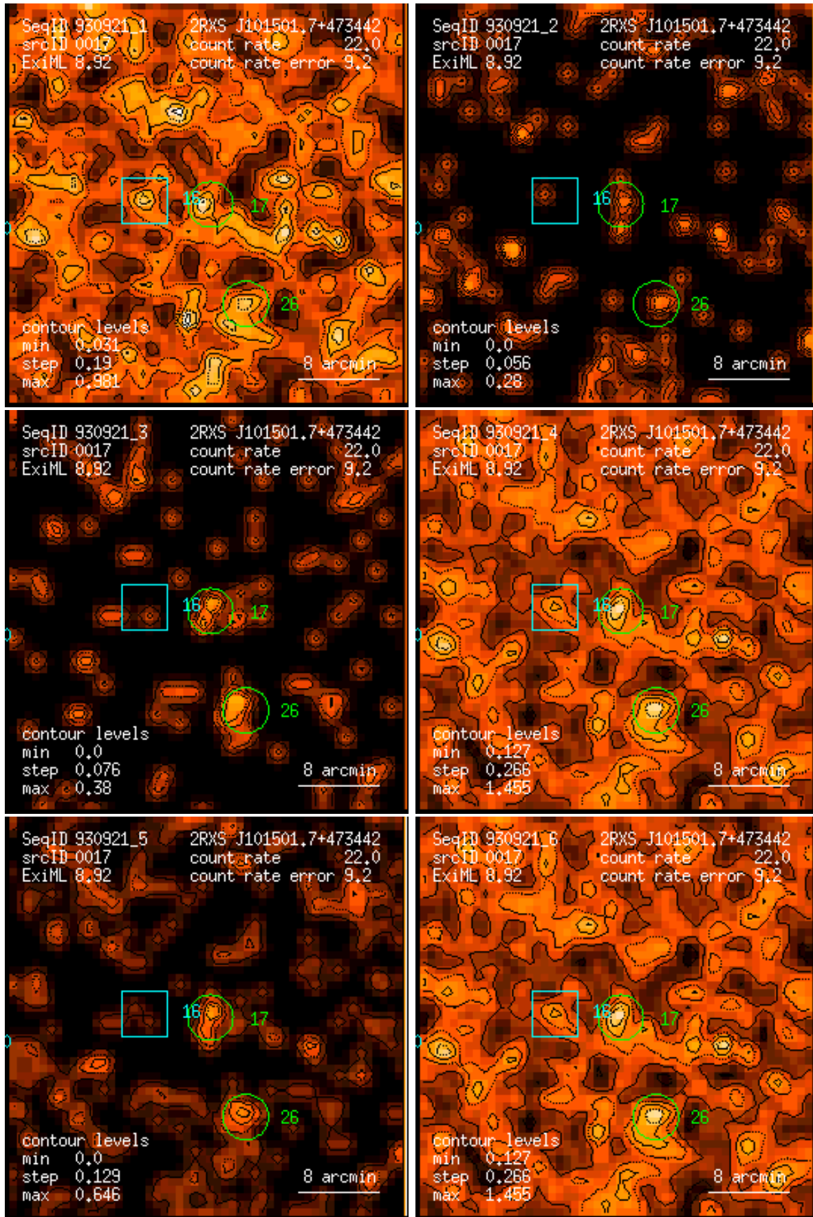
Figure 17: RASS 930921: detection 0017: band rate images, Gaussian filter: (1) PSPC channels 11 – 41, (2) 52 – 90, (3) 91 – 201, (4) 11 – 235, (5) 52 – 201, (6) 11 – 201. Broad band rates in counts/ks. Band rate contour levels in counts/ks/arcmin 2 .
