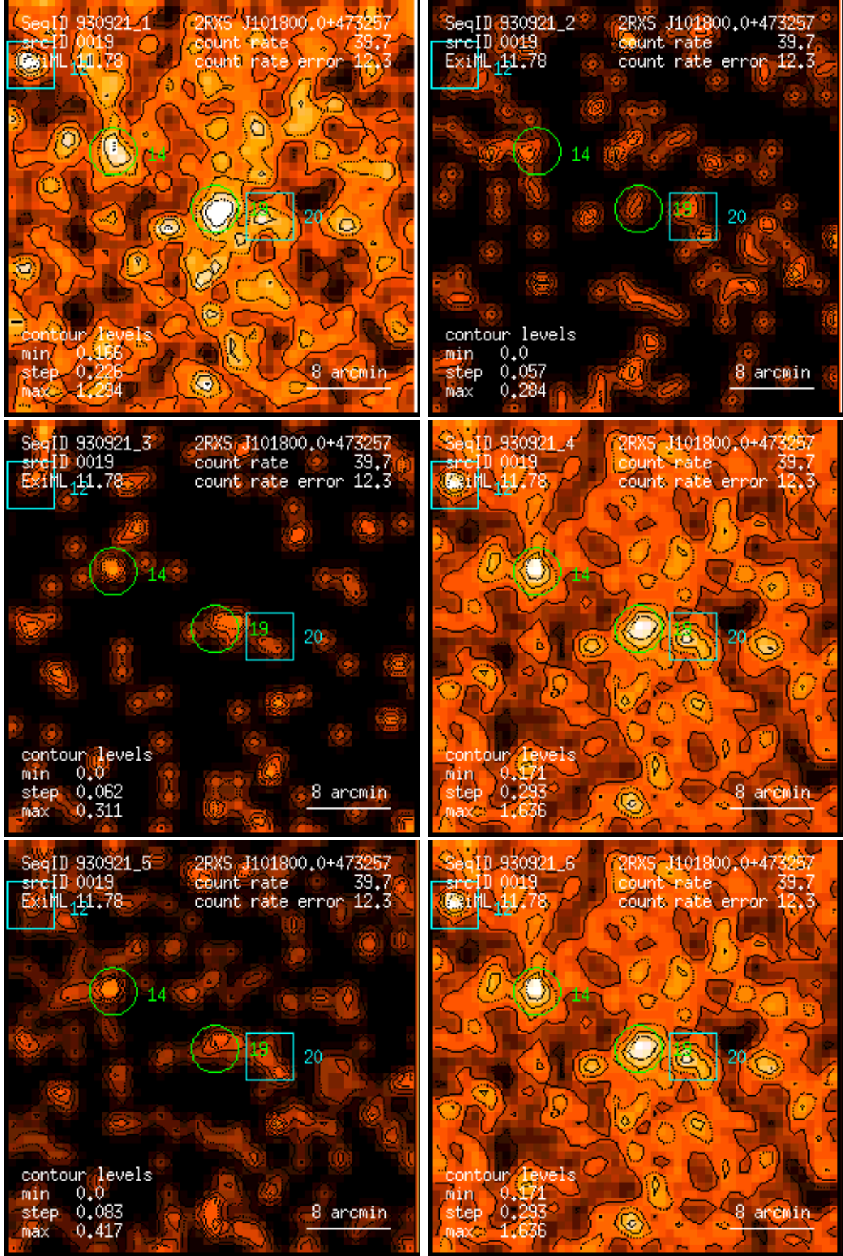
Figure 19: RASS 930921: detection 0019: band rate images, Gaussian filter: (1) PSPC channels 11 – 41, (2) 52 – 90, (3) 91 – 201, (4) 11 – 235, (5) 52 – 201, (6) 11 – 201. Broad band rates in counts/ks. Band rate contour levels in counts/ks/arcmin 2 .
