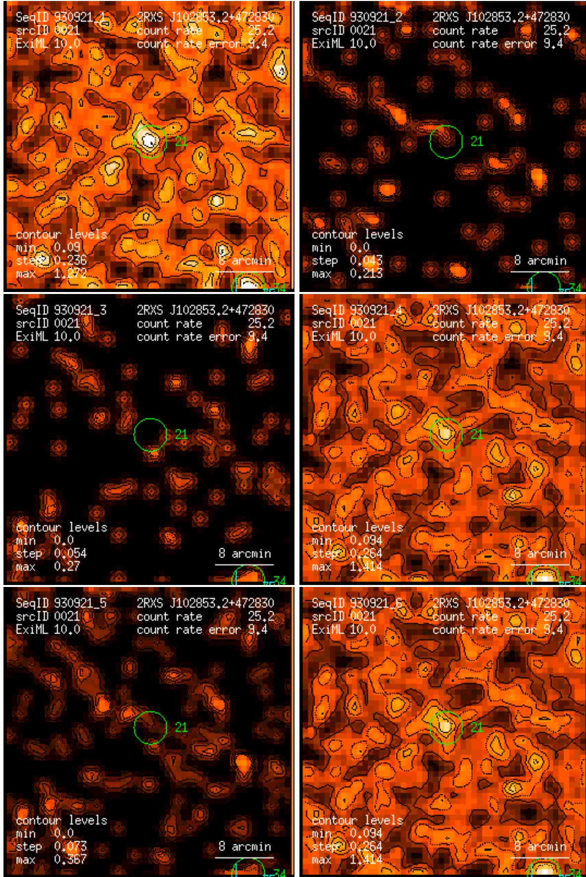
Figure 21: RASS 930921: detection 0021: band rate images, Gaussian filter: (1) PSPC channels 11 – 41, (2) 52 – 90, (3) 91 – 201, (4) 11 – 235, (5) 52 – 201, (6) 11 – 201. Broad band rates in counts/ks. Band rate contour levels in counts/ks/arcmin 2 .
