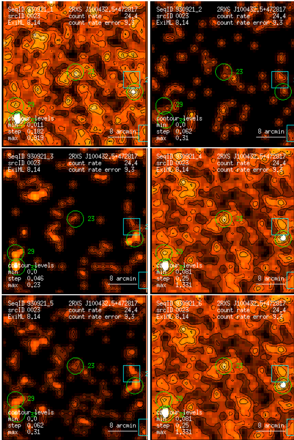
Figure 23: RASS 930921: detection 0023: band rate images, Gaussian filter: (1) PSPC channels 11 – 41, (2) 52 – 90, (3) 91 – 201, (4) 11 – 235, (5) 52 – 201, (6) 11 – 201. Broad band rates in counts/ks. Band rate contour levels in counts/ks/arcmin 2 .
