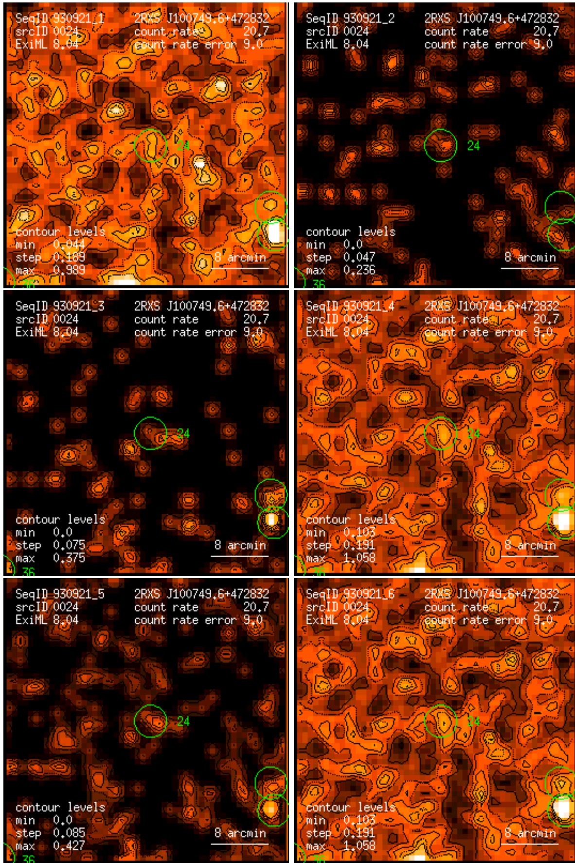
Figure 24: RASS 930921: detection 0024: band rate images, Gaussian filter: (1) PSPC channels 11 – 41, (2) 52 – 90, (3) 91 – 201, (4) 11 – 235, (5) 52 – 201, (6) 11 – 201. Broad band rates in counts/ks. Band rate contour levels in counts/ks/arcmin 2 .
