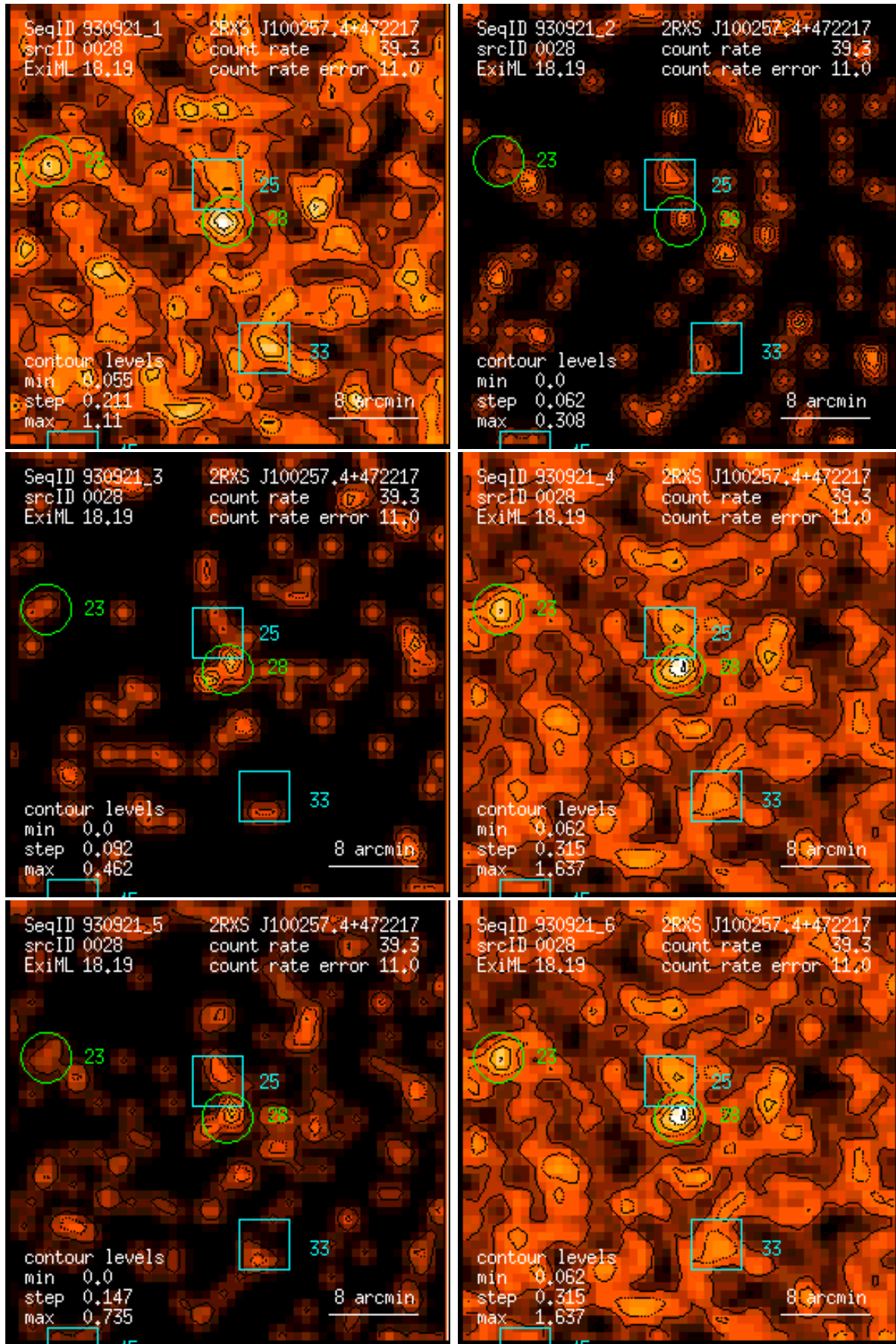
Figure 28: RASS 930921: detection 0028: band rate images, Gaussian filter: (1) PSPC channels 11 – 41, (2) 52 – 90, (3) 91 – 201, (4) 11 – 235, (5) 52 – 201, (6) 11 – 201. Broad band rates in counts/ks. Band rate contour levels in counts/ks/arcmin 2 .
