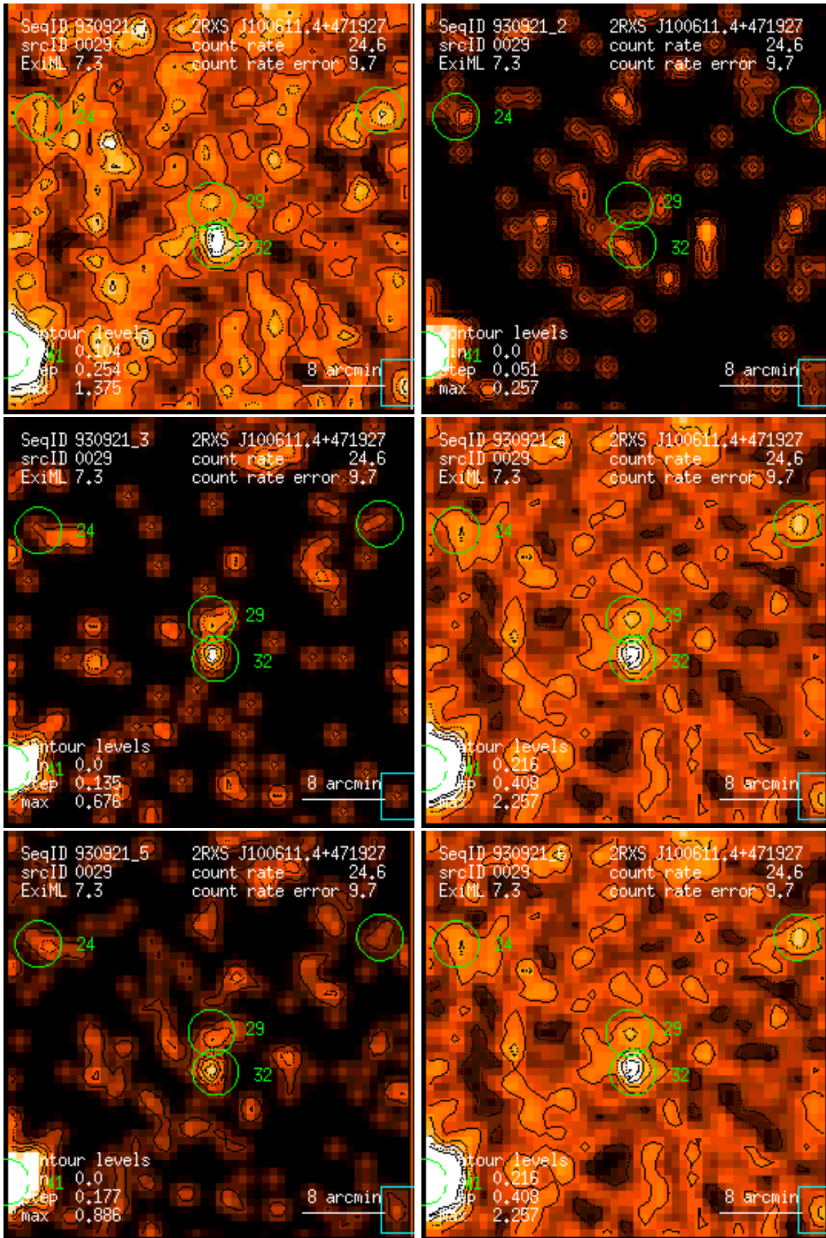
Figure 29: RASS 930921: detection 0029: band rate images, Gaussian filter: (1) PSPC channels 11 – 41, (2) 52 – 90, (3) 91 – 201, (4) 11 – 235, (5) 52 – 201, (6) 11 – 201. Broad band rates in counts/ks. Band rate contour levels in counts/ks/arcmin 2 .
