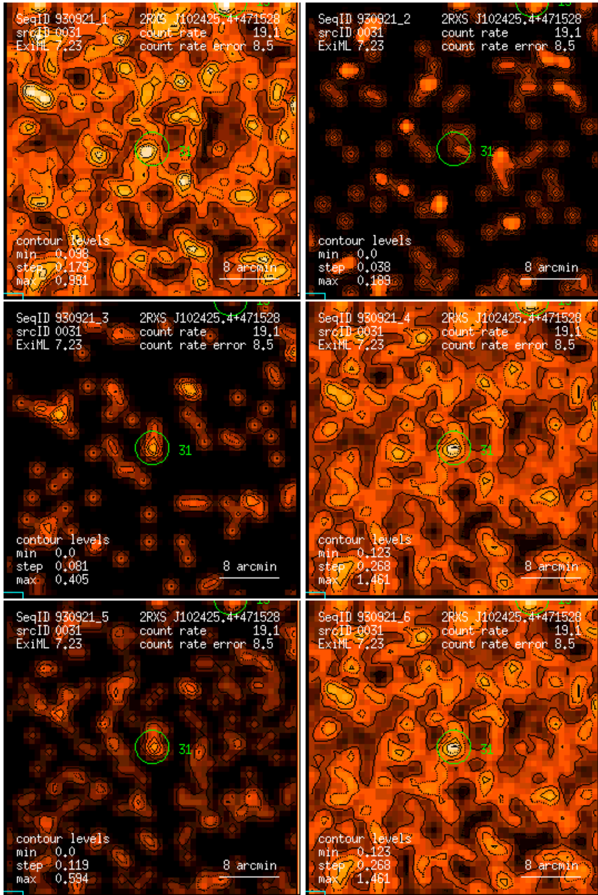
Figure 31: RASS 930921: detection 0031: band rate images, Gaussian filter: (1) PSPC channels 11 – 41, (2) 52 – 90, (3) 91 – 201, (4) 11 – 235, (5) 52 – 201, (6) 11 – 201. Broad band rates in counts/ks. Band rate contour levels in counts/ks/arcmin 2 .
