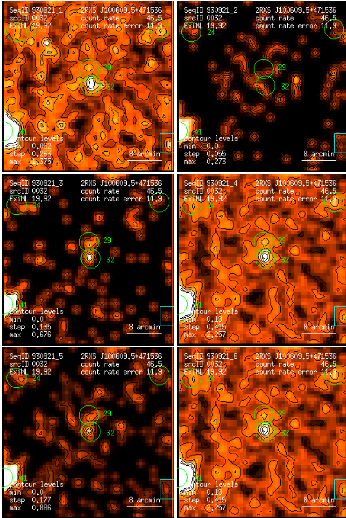
Figure 32: RASS 930921: detection 0032: band rate images, Gaussian filter: (1) PSPC channels 11 – 41, (2) 52 – 90, (3) 91 – 201, (4) 11 – 235, (5) 52 – 201, (6) 11 – 201. Broad band rates in counts/ks. Band rate contour levels in counts/ks/arcmin 2 .
