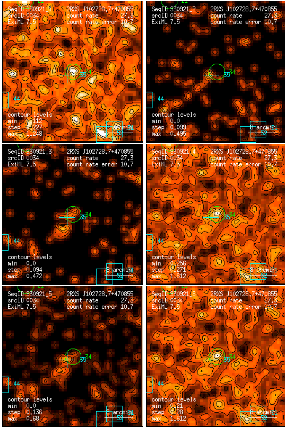
Figure 34: RASS 930921: detection 0034: band rate images, Gaussian filter: (1) PSPC channels 11 – 41, (2) 52 – 90, (3) 91 – 201, (4) 11 – 235, (5) 52 – 201, (6) 11 – 201. Broad band rates in counts/ks. Band rate contour levels in counts/ks/arcmin 2 .
