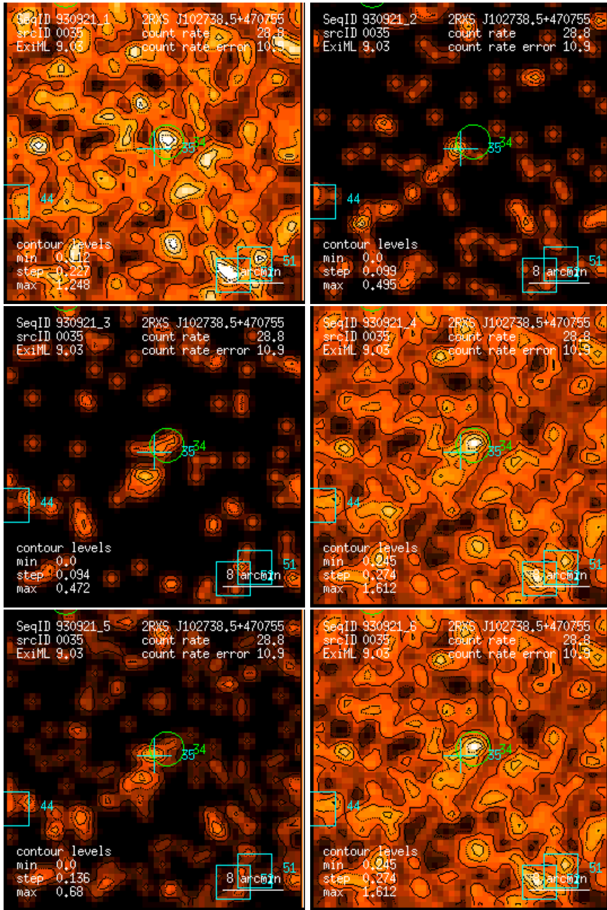
Figure 35: RASS 930921: detection 0035: band rate images, Gaussian filter: (1) PSPC channels 11 – 41, (2) 52 – 90, (3) 91 – 201, (4) 11 – 235, (5) 52 – 201, (6) 11 – 201. Broad band rates in counts/ks. Band rate contour levels in counts/ks/arcmin 2 .
