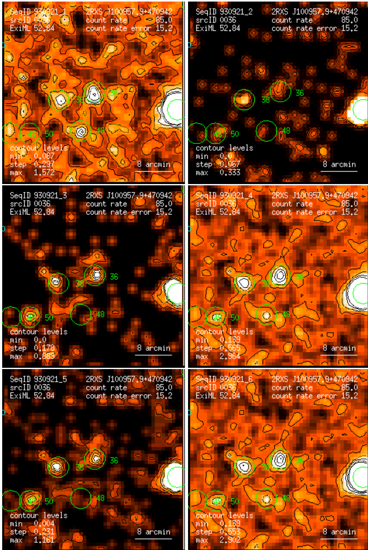
Figure 36: RASS 930921: detection 0036: band rate images, Gaussian filter: (1) PSPC channels 11 – 41, (2) 52 – 90, (3) 91 – 201, (4) 11 – 235, (5) 52 – 201, (6) 11 – 201. Broad band rates in counts/ks. Band rate contour levels in counts/ks/arcmin 2 .
