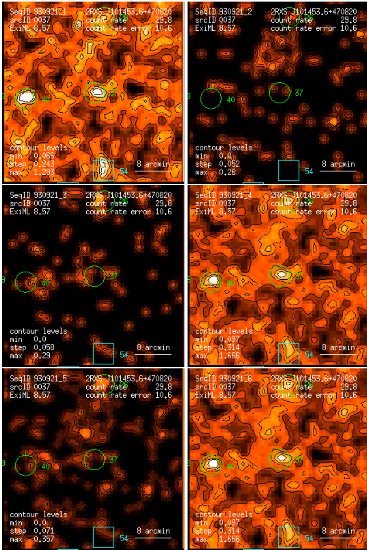
Figure 37: RASS 930921: detection 0037: band rate images, Gaussian filter: (1) PSPC channels 11 – 41, (2) 52 – 90, (3) 91 – 201, (4) 11 – 235, (5) 52 – 201, (6) 11 – 201. Broad band rates in counts/ks. Band rate contour levels in counts/ks/arcmin 2 .
