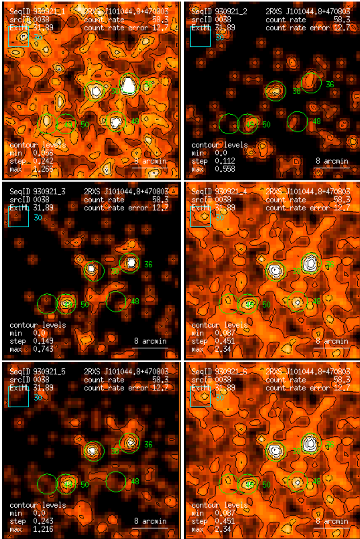
Figure 38: RASS 930921: detection 0038: band rate images, Gaussian filter: (1) PSPC channels 11 – 41, (2) 52 – 90, (3) 91 – 201, (4) 11 – 235, (5) 52 – 201, (6) 11 – 201. Broad band rates in counts/ks. Band rate contour levels in counts/ks/arcmin 2 .
