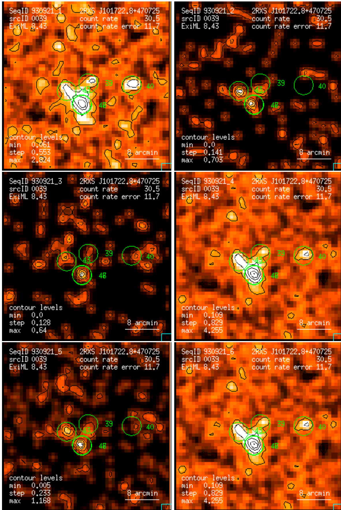
Figure 39: RASS 930921: detection 0039: band rate images, Gaussian filter: (1) PSPC channels 11 – 41, (2) 52 – 90, (3) 91 – 201, (4) 11 – 235, (5) 52 – 201, (6) 11 – 201. Broad band rates in counts/ks. Band rate contour levels in counts/ks/arcmin 2 .
