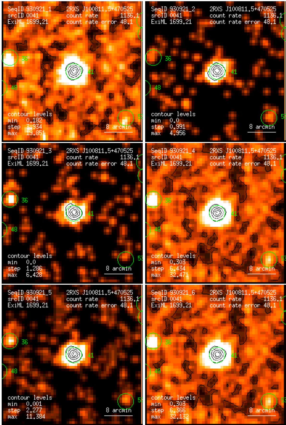
Figure 41: RASS 930921: detection 0041: band rate images, Gaussian filter: (1) PSPC channels 11 – 41, (2) 52 – 90, (3) 91 – 201, (4) 11 – 235, (5) 52 – 201, (6) 11 – 201. Broad band rates in counts/ks. Band rate contour levels in counts/ks/arcmin 2 .
