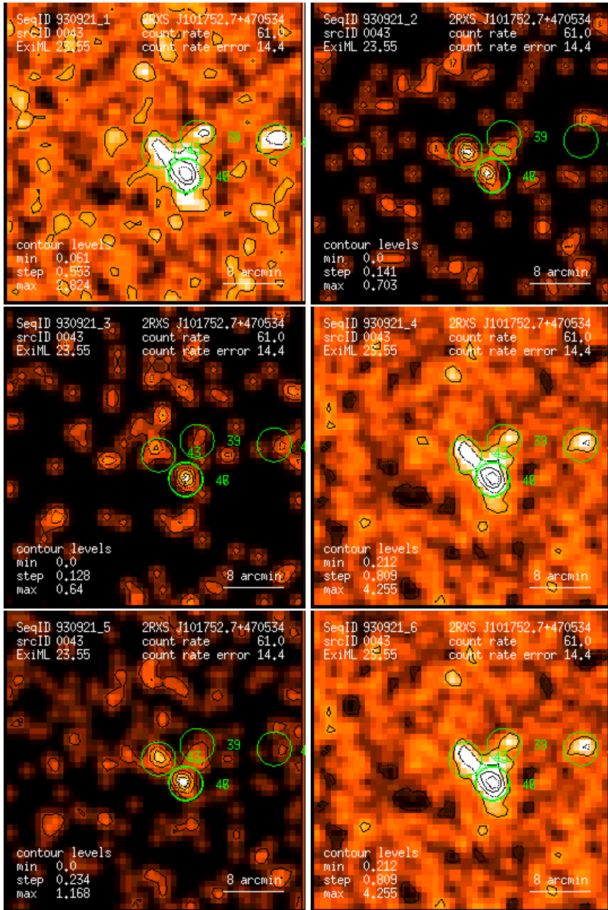
Figure 43: RASS 930921: detection 0043: band rate images, Gaussian filter: (1) PSPC channels 11 – 41, (2) 52 – 90, (3) 91 – 201, (4) 11 – 235, (5) 52 – 201, (6) 11 – 201. Broad band rates in counts/ks. Band rate contour levels in counts/ks/arcmin 2 .
