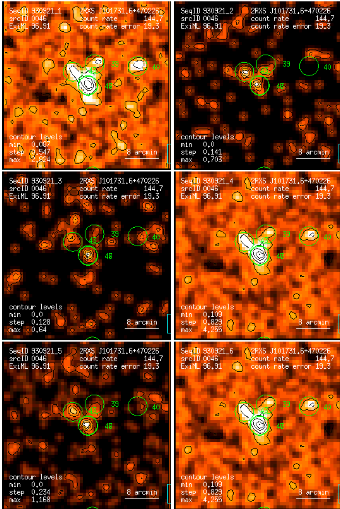
Figure 46: RASS 930921: detection 0046: band rate images, Gaussian filter: (1) PSPC channels 11 – 41, (2) 52 – 90, (3) 91 – 201, (4) 11 – 235, (5) 52 – 201, (6) 11 – 201. Broad band rates in counts/ks. Band rate contour levels in counts/ks/arcmin 2 .
