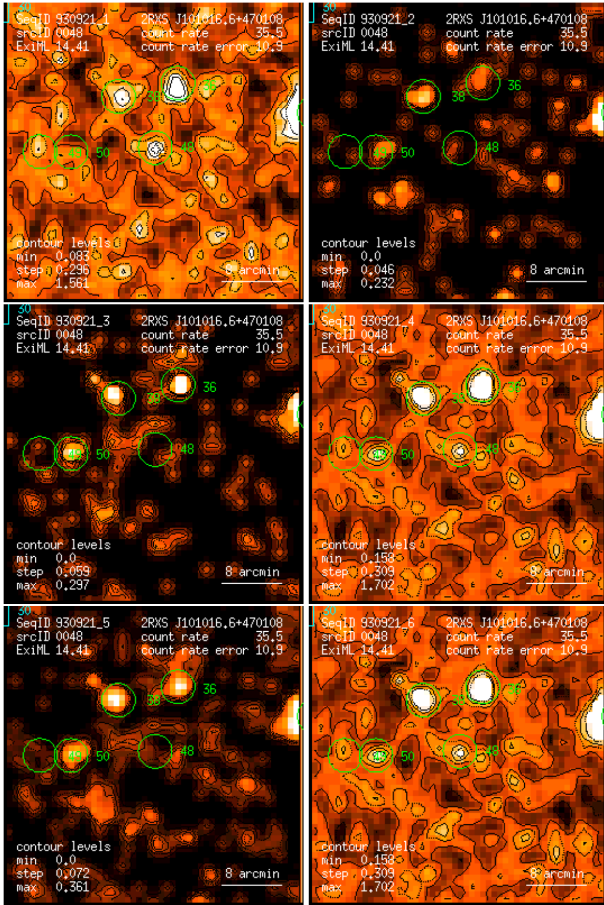
Figure 48: RASS 930921: detection 0048: band rate images, Gaussian filter: (1) PSPC channels 11 – 41, (2) 52 – 90, (3) 91 – 201, (4) 11 – 235, (5) 52 – 201, (6) 11 – 201. Broad band rates in counts/ks. Band rate contour levels in counts/ks/arcmin 2 .
