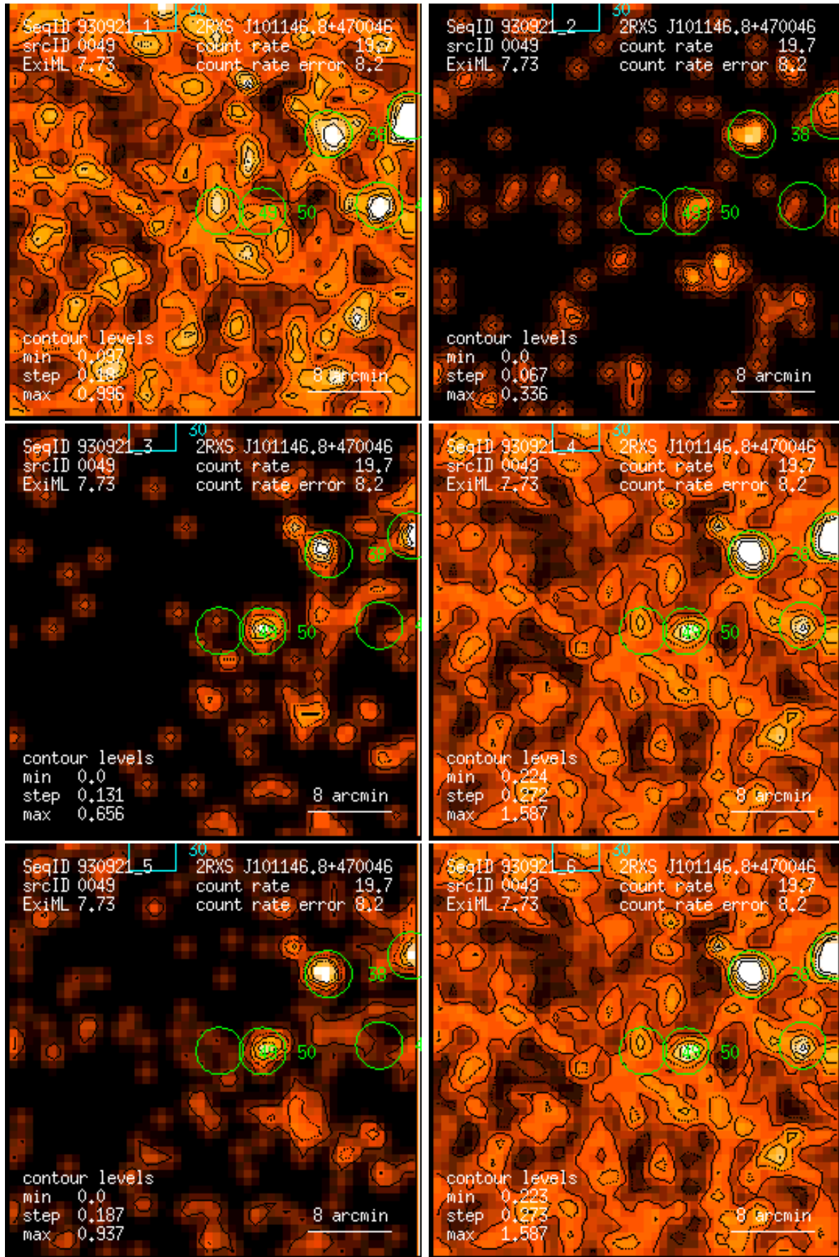
Figure 49: RASS 930921: detection 0049: band rate images, Gaussian filter: (1) PSPC channels 11 – 41, (2) 52 – 90, (3) 91 – 201, (4) 11 – 235, (5) 52 – 201, (6) 11 – 201. Broad band rates in counts/ks. Band rate contour levels in counts/ks/arcmin 2 .
