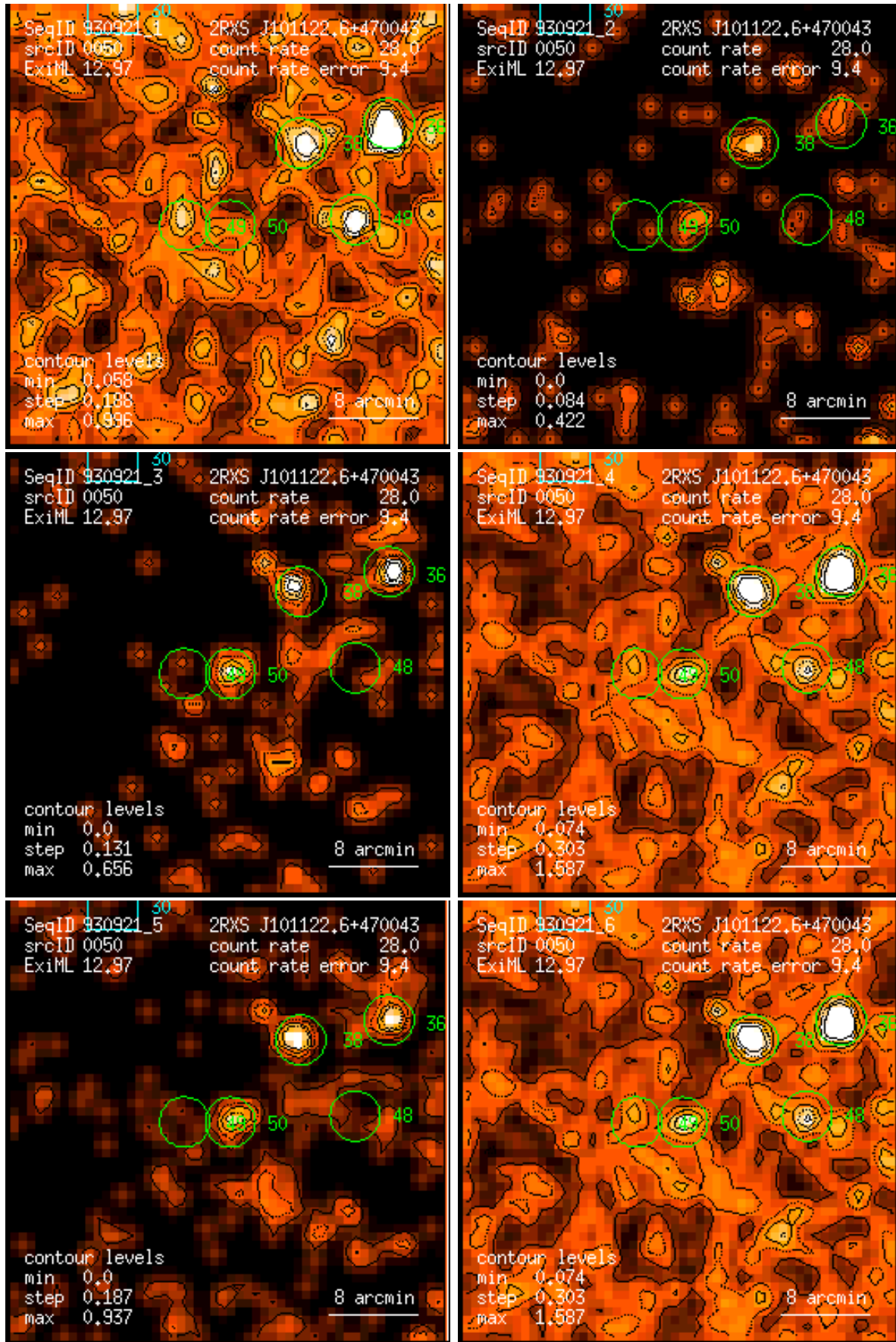
Figure 50: RASS 930921: detection 0050: band rate images, Gaussian filter: (1) PSPC channels 11 – 41, (2) 52 – 90, (3) 91 – 201, (4) 11 – 235, (5) 52 – 201, (6) 11 – 201. Broad band rates in counts/ks. Band rate contour levels in counts/ks/arcmin 2 .
