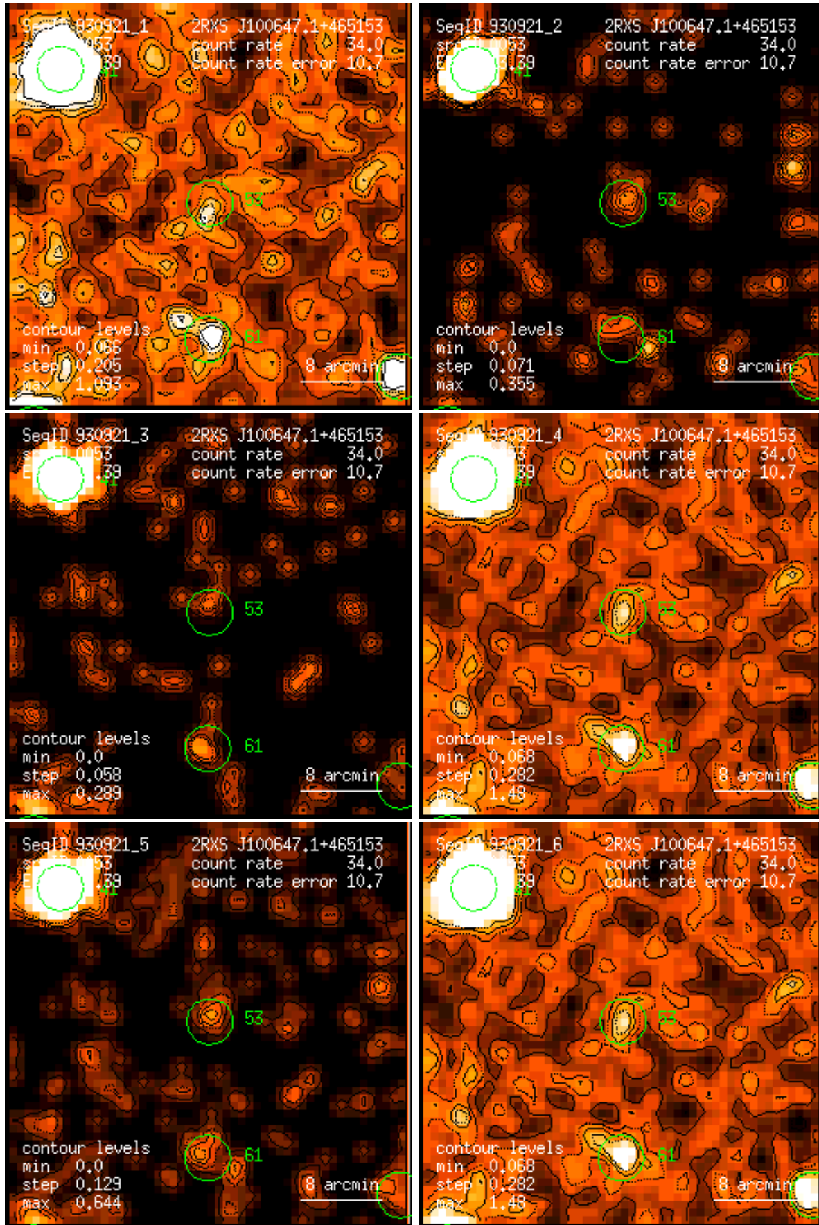
Figure 53: RASS 930921: detection 0053: band rate images, Gaussian filter: (1) PSPC channels 11 – 41, (2) 52 – 90, (3) 91 – 201, (4) 11 – 235, (5) 52 – 201, (6) 11 – 201. Broad band rates in counts/ks. Band rate contour levels in counts/ks/arcmin 2 .
