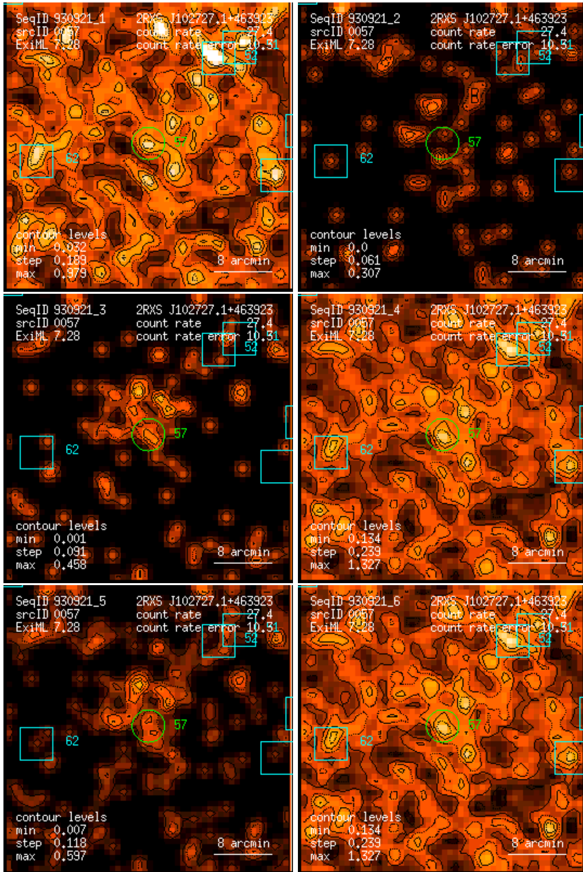
Figure 57: RASS 930921: detection 0057: band rate images, Gaussian filter: (1) PSPC channels 11 – 41, (2) 52 – 90, (3) 91 – 201, (4) 11 – 235, (5) 52 – 201, (6) 11 – 201. Broad band rates in counts/ks. Band rate contour levels in counts/ks/arcmin 2 .
