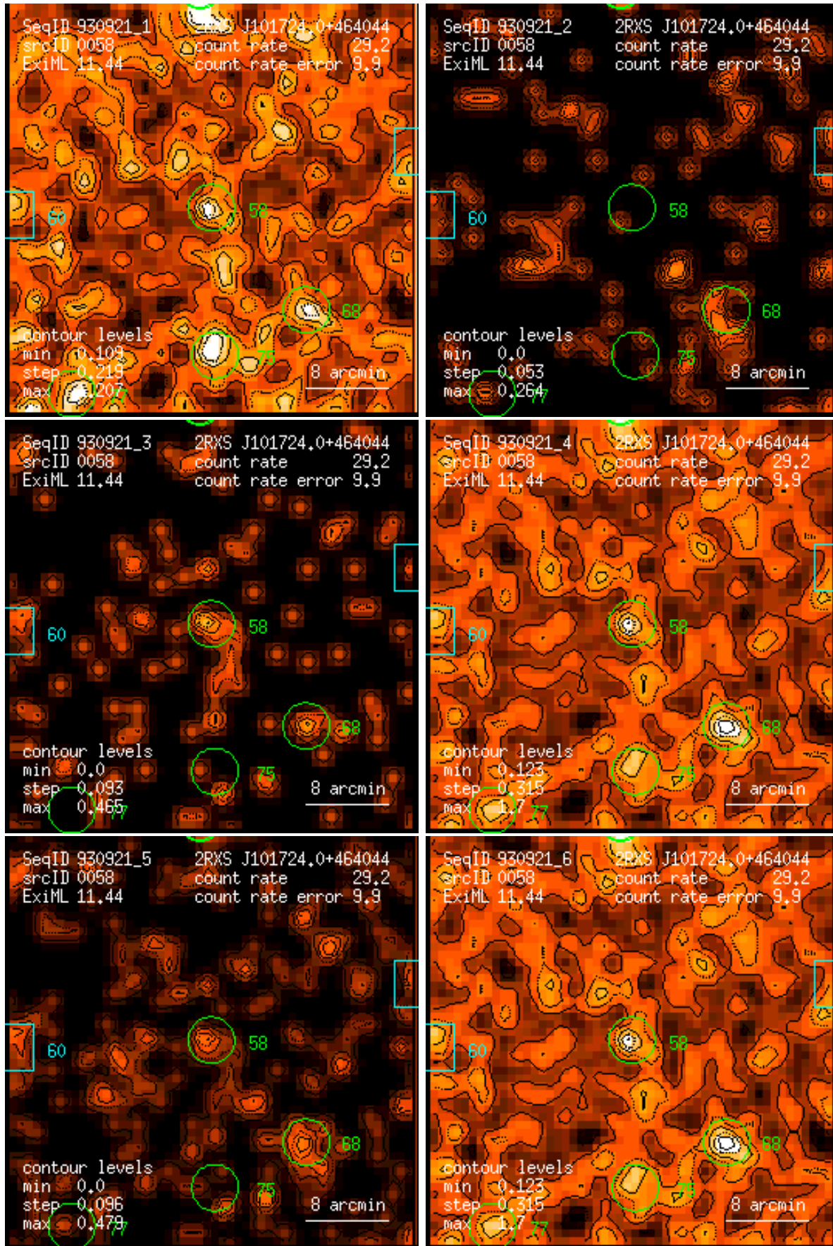
Figure 58: RASS 930921: detection 0058: band rate images, Gaussian filter: (1) PSPC channels 11 – 41, (2) 52 – 90, (3) 91 – 201, (4) 11 – 235, (5) 52 – 201, (6) 11 – 201. Broad band rates in counts/ks. Band rate contour levels in counts/ks/arcmin 2 .
