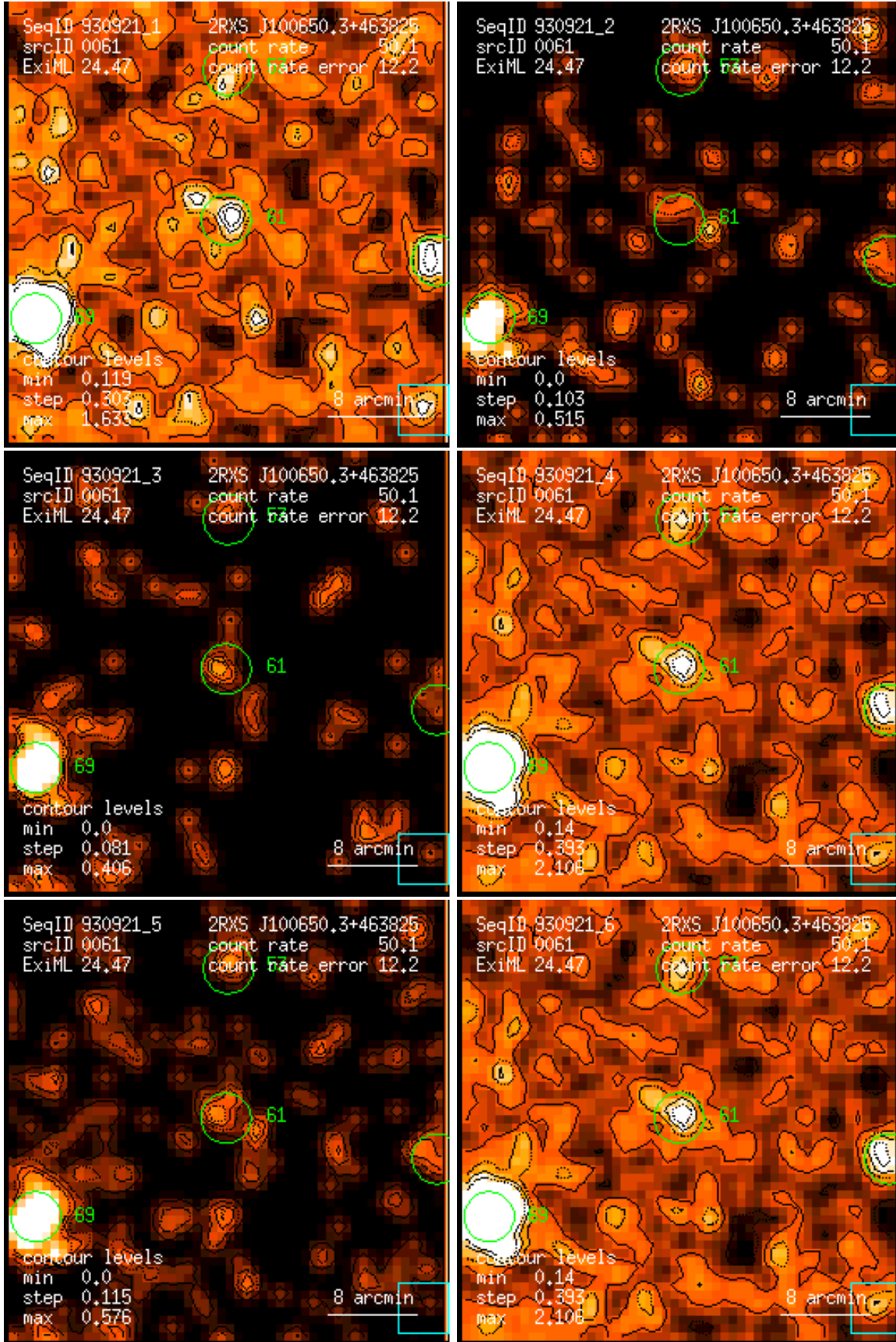
Figure 61: RASS 930921: detection 0061: band rate images, Gaussian filter: (1) PSPC channels 11 – 41, (2) 52 – 90, (3) 91 – 201, (4) 11 – 235, (5) 52 – 201, (6) 11 – 201. Broad band rates in counts/ks. Band rate contour levels in counts/ks/arcmin 2 .
