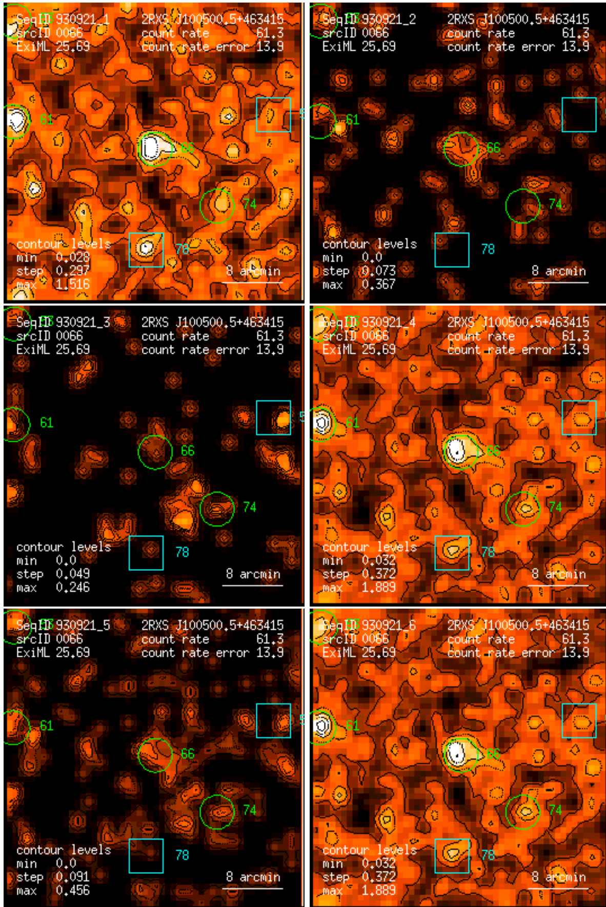
Figure 66: RASS 930921: detection 0066: band rate images, Gaussian filter: (1) PSPC channels 11 – 41, (2) 52 – 90, (3) 91 – 201, (4) 11 – 235, (5) 52 – 201, (6) 11 – 201. Broad band rates in counts/ks. Band rate contour levels in counts/ks/arcmin 2 .
