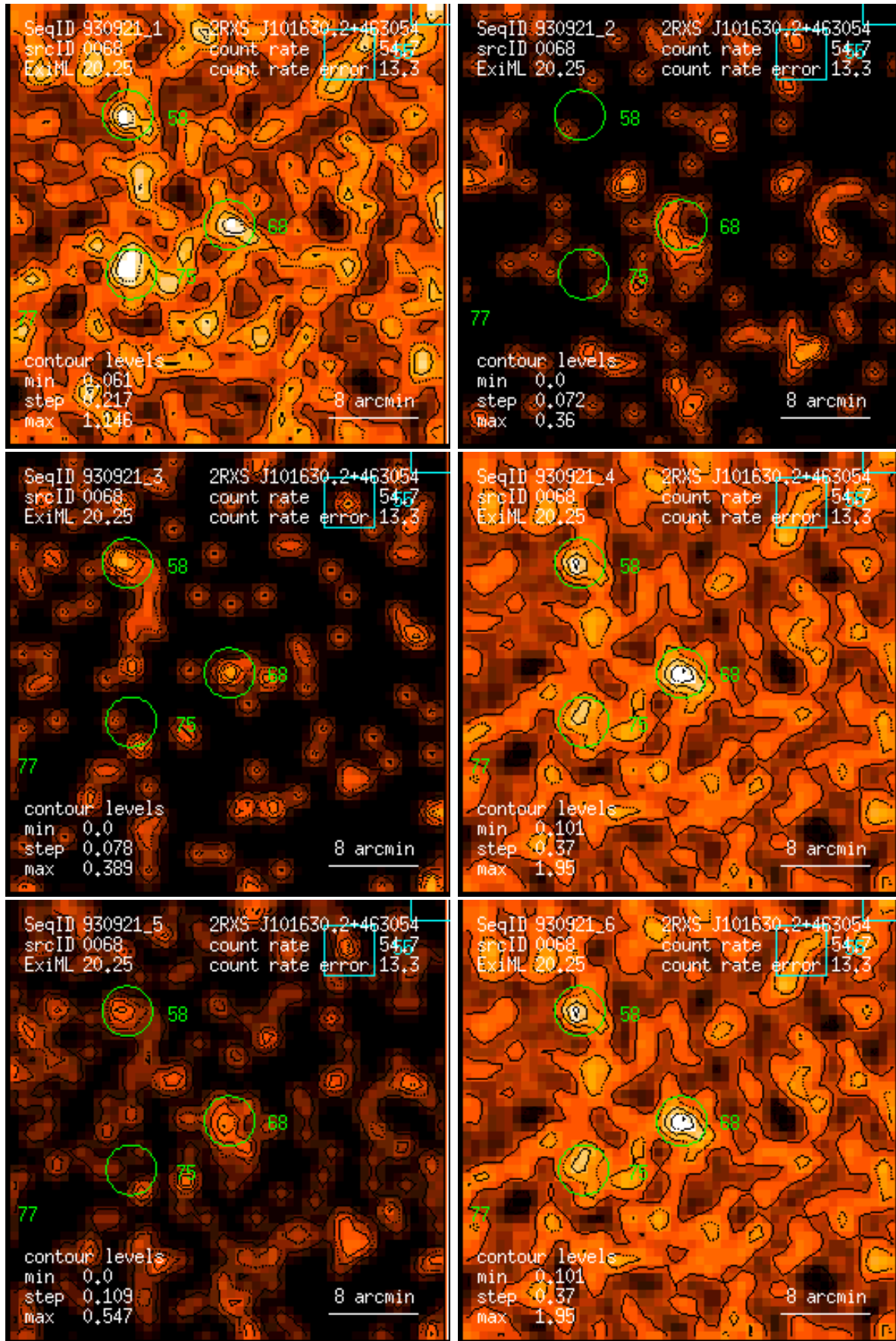
Figure 68: RASS 930921: detection 0068: band rate images, Gaussian filter: (1) PSPC channels 11 – 41, (2) 52 – 90, (3) 91 – 201, (4) 11 – 235, (5) 52 – 201, (6) 11 – 201. Broad band rates in counts/ks. Band rate contour levels in counts/ks/arcmin 2 .
