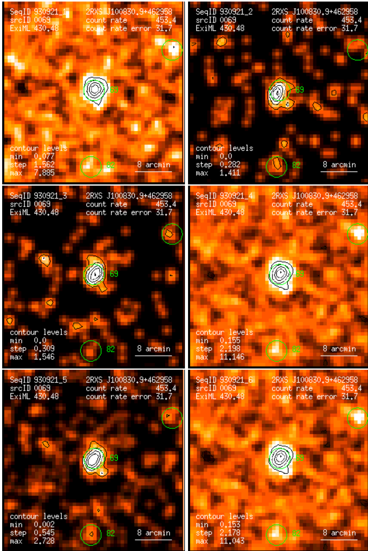
Figure 69: RASS 930921: detection 0069: band rate images, Gaussian filter: (1) PSPC channels 11 – 41, (2) 52 – 90, (3) 91 – 201, (4) 11 – 235, (5) 52 – 201, (6) 11 – 201. Broad band rates in counts/ks. Band rate contour levels in counts/ks/arcmin 2 .
