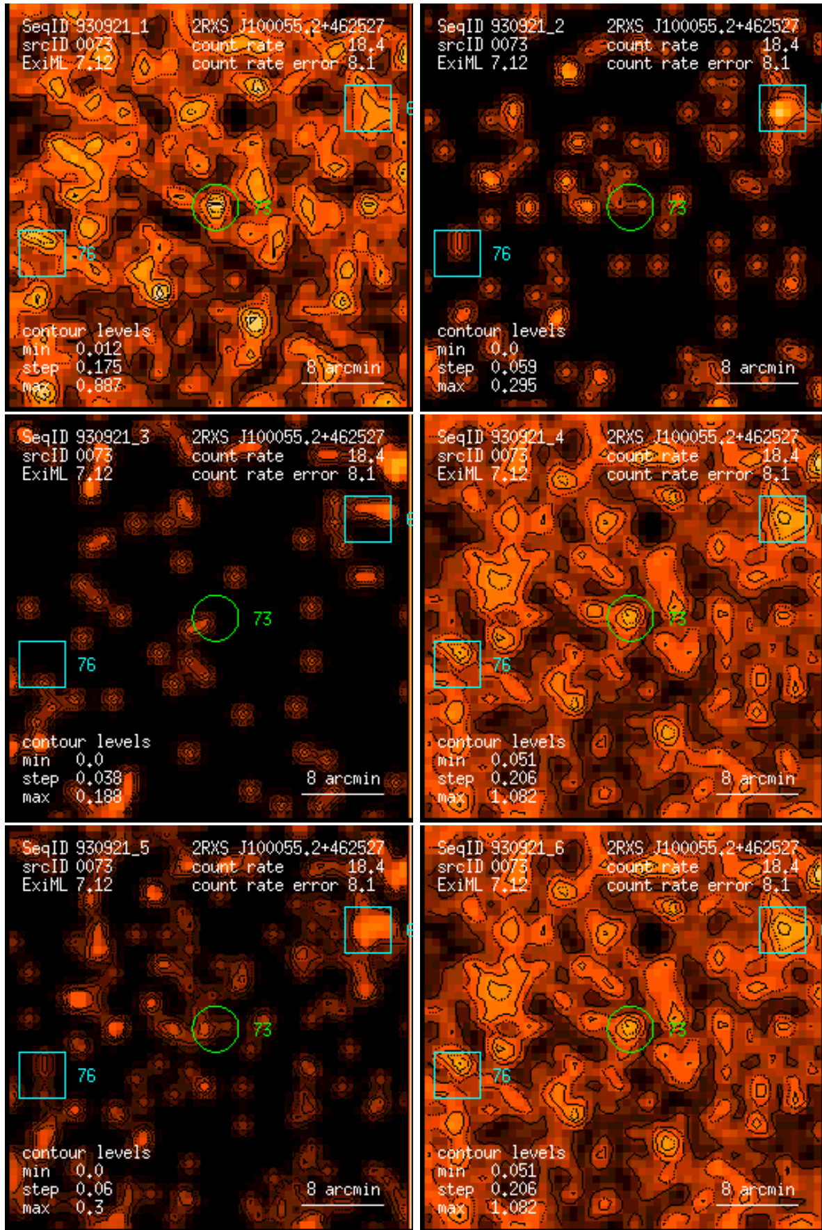
Figure 73: RASS 930921: detection 0073: band rate images, Gaussian filter: (1) PSPC channels 11 – 41, (2) 52 – 90, (3) 91 – 201, (4) 11 – 235, (5) 52 – 201, (6) 11 – 201. Broad band rates in counts/ks. Band rate contour levels in counts/ks/arcmin 2 .
