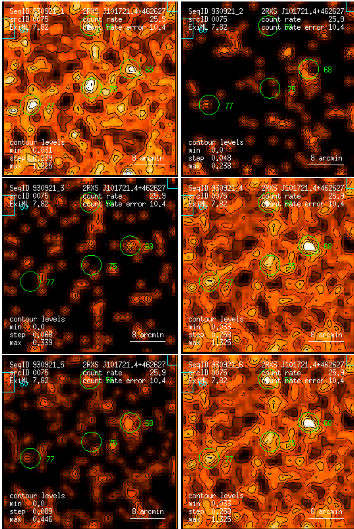
Figure 75: RASS 930921: detection 0075: band rate images, Gaussian filter: (1) PSPC channels 11 – 41, (2) 52 – 90, (3) 91 – 201, (4) 11 – 235, (5) 52 – 201, (6) 11 – 201. Broad band rates in counts/ks. Band rate contour levels in counts/ks/arcmin 2 .
