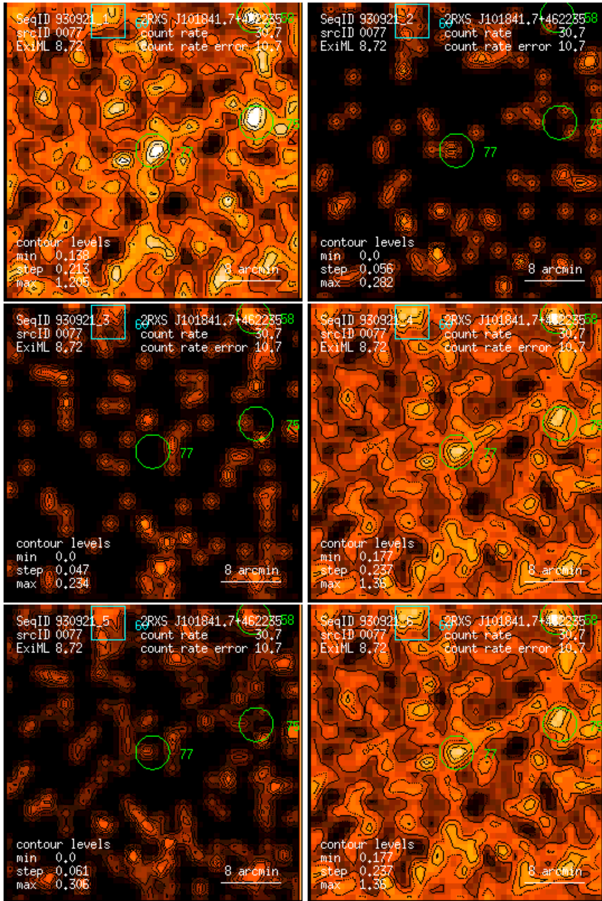
Figure 77: RASS 930921: detection 0077: band rate images, Gaussian filter: (1) PSPC channels 11 – 41, (2) 52 – 90, (3) 91 – 201, (4) 11 – 235, (5) 52 – 201, (6) 11 – 201. Broad band rates in counts/ks. Band rate contour levels in counts/ks/arcmin 2 .
