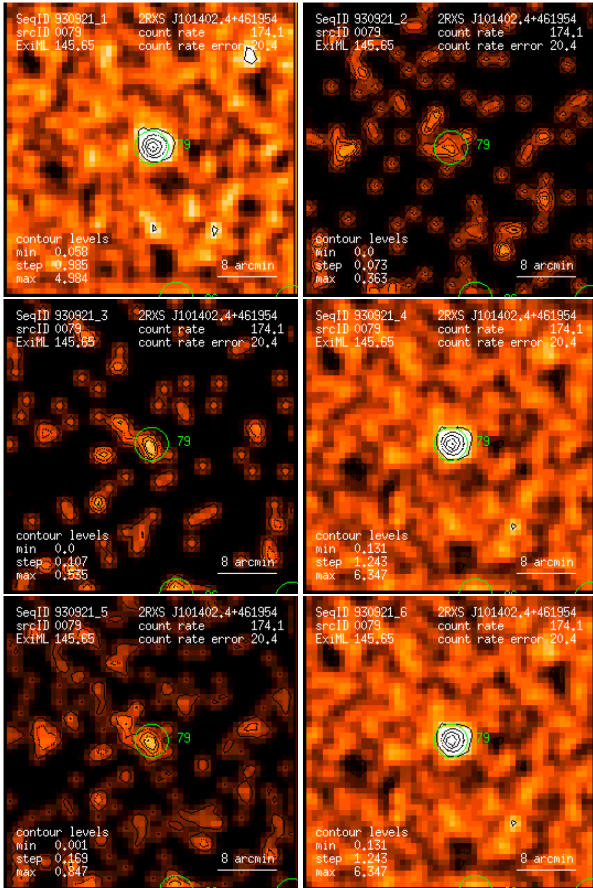
Figure 79: RASS 930921: detection 0079: band rate images, Gaussian filter: (1) PSPC channels 11 – 41, (2) 52 – 90, (3) 91 – 201, (4) 11 – 235, (5) 52 – 201, (6) 11 – 201. Broad band rates in counts/ks. Band rate contour levels in counts/ks/arcmin 2 .
